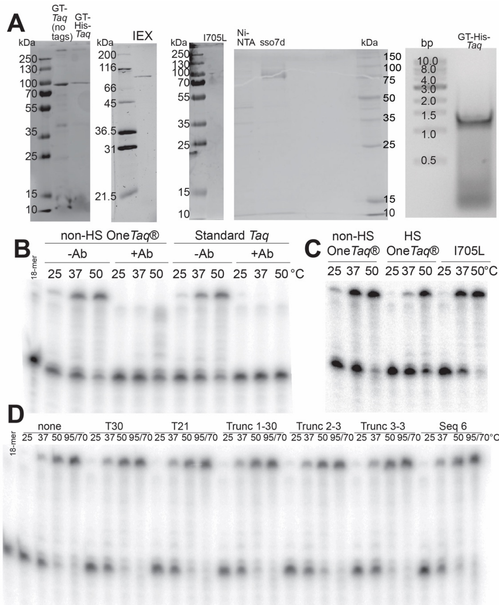
Supp Figure S4. Purification and activity of GT-Taq. (A) SDS-PAGE (12% polyacrylamide with Coomassie-staining or using Bio-Rad stain-free gel imaging) analysis of purified GT-His-Taq (94 kDa) after Ni-NTA column and ion exchange (IEX) chromatography, I705L Taq variant (94 kDa), and sso7d-Taq fusion after Ni-NTA purification (102 kDa). Right, 1.2% agarose gel showing DNA polymerase activity of GT-His-Taq. (B) Effect of Platinum® Taq monoclonal antibody (Thermo Fisher Scientific #10965-028) on two non-HS commercial DNA polymerases: OneTaq® (NEB #M0480) and standard Taq (NEB #M0273). (C) Polymerization by different DNA polymerases as a function of incubation temperature: non-hot-start (HS) OneTaq® (NEB #M0480); HS (aptamer-based) OneTaq® (NEB #M0481); I705L (mutant Taq). (D) Effect of six aptamers (see Supp Table S4 for sequences) on non-HS OneTaq® (NEB #M0480).
