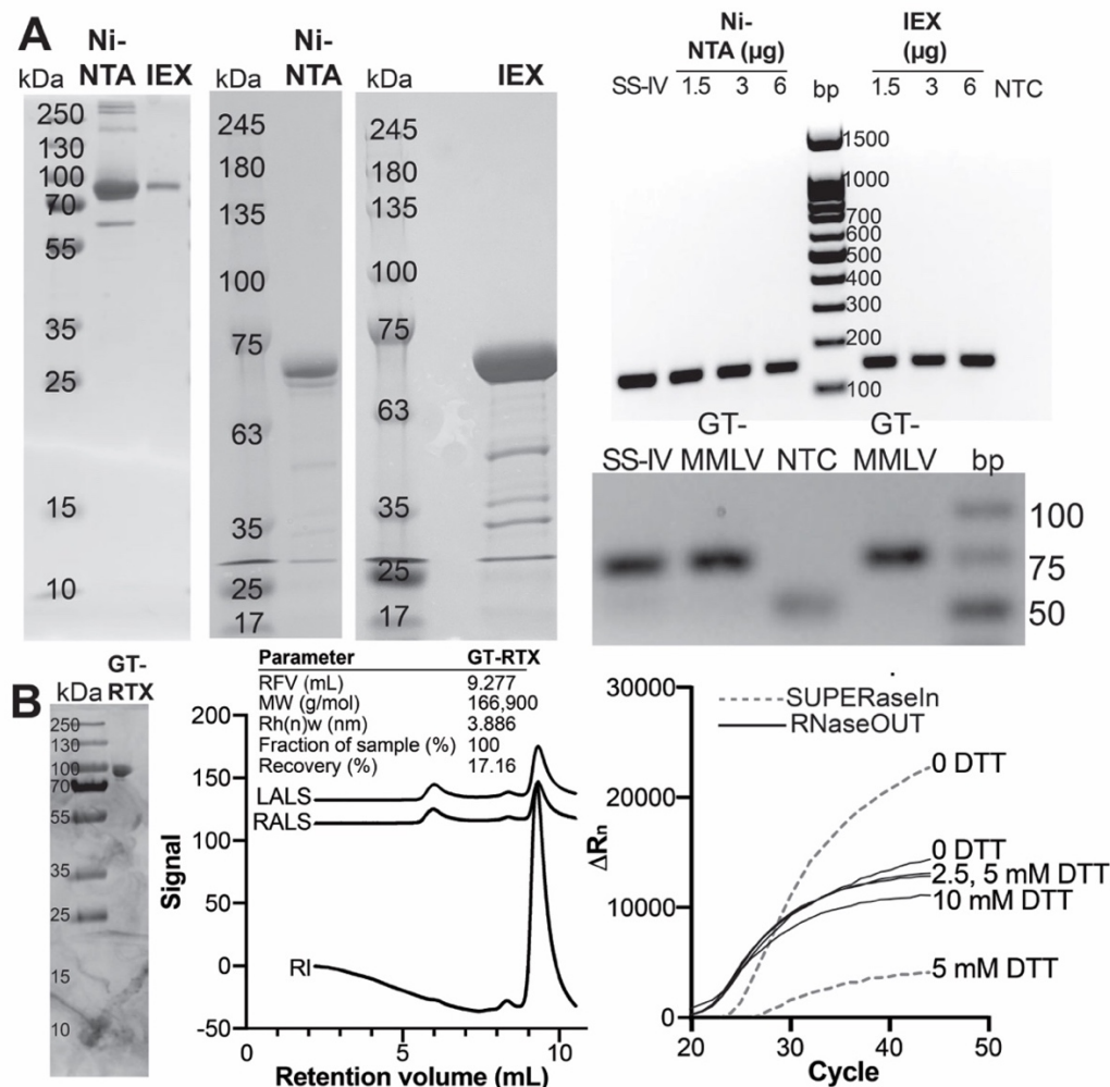
Supp Figure S3. Purification, activity, and characteristics of GT-MMLV M5 RT and GT-RTX reverse transcriptases. (A) Top left : Purified His-tagged GT-MMLV (12% SDS-PAGE, expected product: 77.8 kDa) from Ni-NTA column and ion exchange (IEX) chromatography. Top gel : 1.5% agarose gel showing reverse transcriptase activity of enzymes from both purification methods at a range of concentrations compared to SuperScript® (SS) IV RT (Thermo Fisher) and no template control (NTC). Only one product was observed at the expected product size of 150 bp. Bottom gel : A 2.0% agarose gel was used to separate RT-PCR products from reactions with SuperScript® (SS) IV RT (Thermo Fisher Scientific) and GT-MMLV, using the CDC N1 primer. The expected size of the N1 amplicon was 72 bp. N1 amplicons are similar in size to primer-dimer in NTC, complicating efforts to assess amplification efficiency by gel electrophoresis. (B) Lower left : Purified GT-RTX (12% SDS-PAGE, expected product: 95 kDa). Middle : OMNISEC results for RTX, calculated based on BSA as a standard, and triple detection using RI, RALS, and LALS detector. Molecular weight was determined using dn/dc based on BSA calculations. Lower right : Effect of DTT (0-10 mM) on RT-qPCR with GT-RTX and Platinum™ II Taq in i) RTX buffer (60 mM Tris-HCl pH 8.4, 25 mM (NH 4 ) 2 SO 4 , 10 mM KCl, 2 mM MgSO 4 ) with SUPERase•In™ RNase inhibitor (Thermo Fisher Scientific #AM2694) or ii) SuperScript® III buffer with RNaseOUT Recombinant Ribonuclease Inhibitor (Thermo Fisher Scientific #10777019). ROX was not included in the RT-qPCR reaction. Cycling conditions were 60 °C for 20 min, 95 °C for 8 min, then 45 cycles of (95 °C for 15s followed by 55 °C for 30s).
