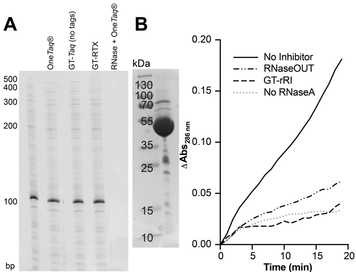
Supp. Figure S5. Purification and RNase inhibition by GT-rRI. (A) Quality control assay for testing RNase A activity. In the ‘positive control’ lane, 1 \mu L of 1 pg/mL RNase A (Thermo Fisher Scientific #EN0531) stock solution was added to OneTaq®. Complete degradation of the RNA ladder was observed, indicating RNase A activity. The other lanes show intact bands with the same intensity with no enzyme, OneTaq®, GT-Taq polymerase, and GT-RTX enzymes, confirming the absence of RNase A in the enzymes. (B) SDS-PAGE analysis of GT-rRI (expected product: 54 kDa) and assay for GT-rRI inhibition of RNaseA-catalyzed cCMP hydrolysis. A reduction in the rate of change in absorbance at 286 nm relative to ‘no inhibitor’ indicates GT-rRI activity.
