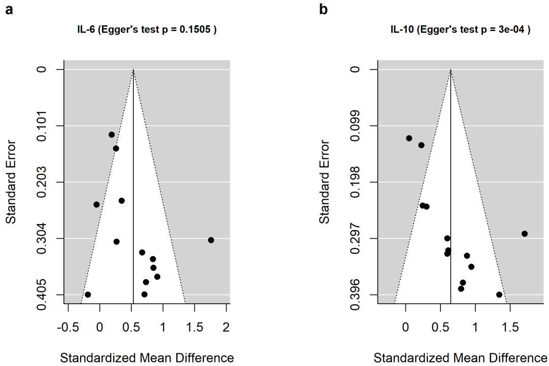
Figure S 2: Funnel plots depicting publication bias in (a) IL-6 and (b) IL-10 meta-analysis
