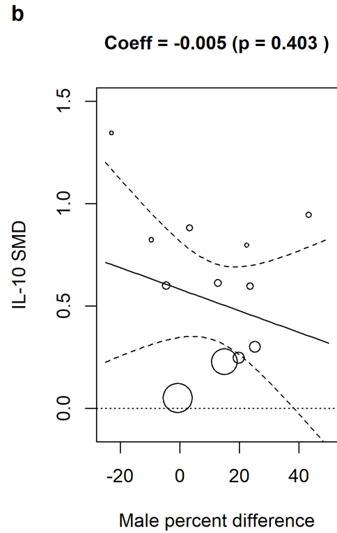
Figure S 1: Meta-regression bubble plots of (a) IL-6 and (b) IL-10 SMD with percent difference of male patients across severe and non-severe groups
