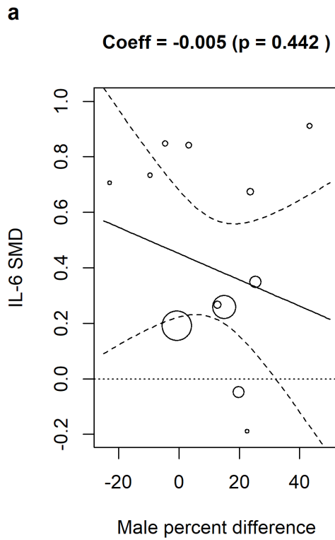
Figure S 1: Meta-regression bubble plots of (a) IL-6 and (b) IL-10 SMD with percent difference of male patients across severe and non-severe groups
