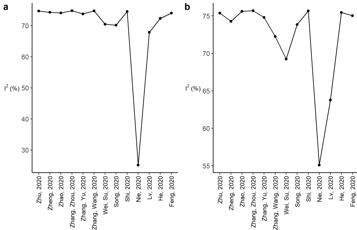
Figure S 3: Sensitivity analysis for (a) IL-6 and (b) IL-10 meta-analysis
