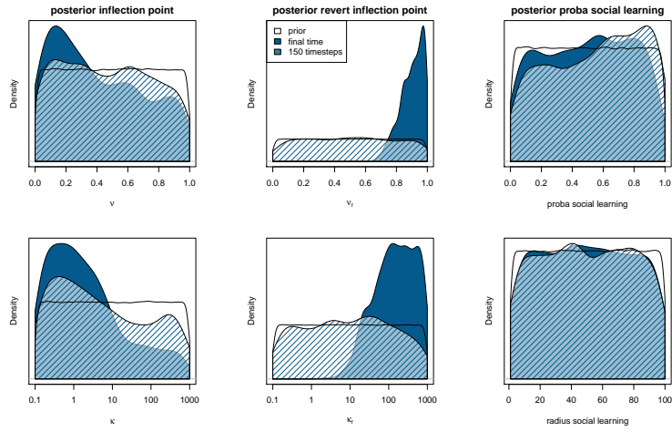
Figure S8: Same than figure 9 but for simulation run with variant E
