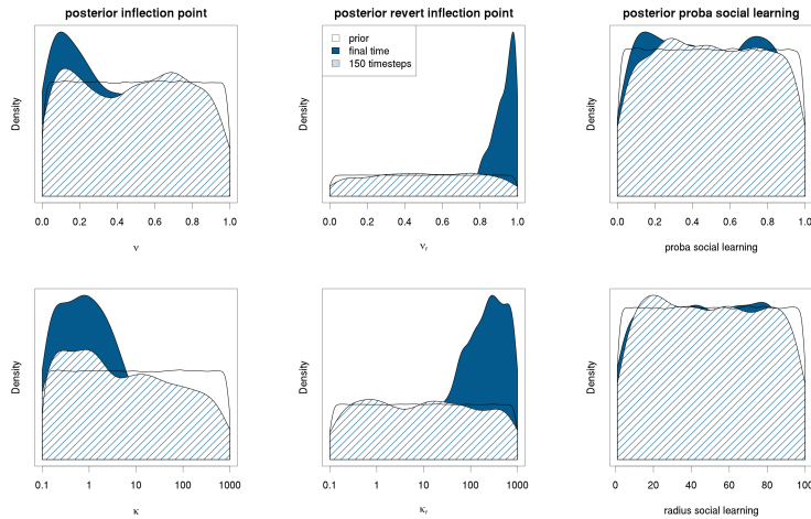
Figure S1: All posterior distributions for the 6 parameters used in our simulations. The white area represents the distribution of the parameters of all simulations (the priors), the blue area represents the distribution for the top 1000 simulations rank using \delta while the shaded area represent the parameters of the 1000 simulations with the lowest number of infected people after 150 timesteps.
