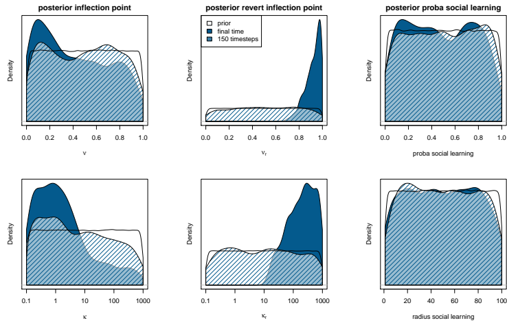
Figure S4: Same than figure 9 but for simulation run with variant A
