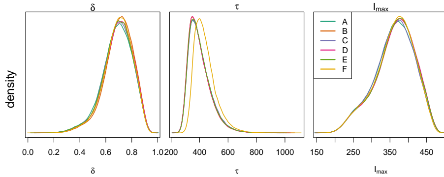
Figure S3: Distribution of the metrics described in the section Results for all simulations for all model (approx 100k simulations per model).
