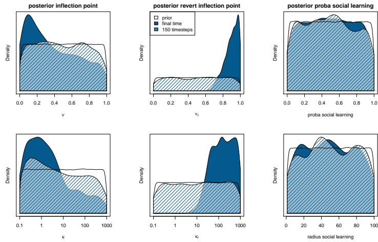
Figure S5: Same than figure 9 but for simulation run with variant B
