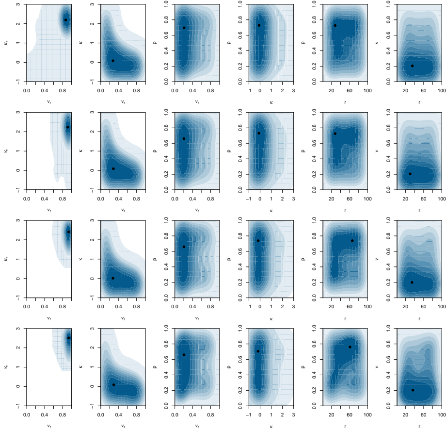
Figure S2: Joint posterior distributions for some combination our 6 parameters. Each distribution represent the parameter distribution of simulation for which the metric \delta is ranked in level respectively 10,000; 12,500; 2,500; 1,000
