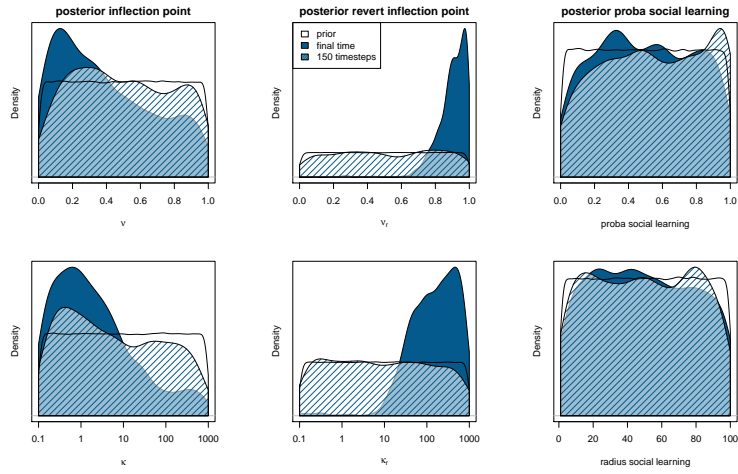
Figure S6: Same than figure 9 but for simulation run with variant C
