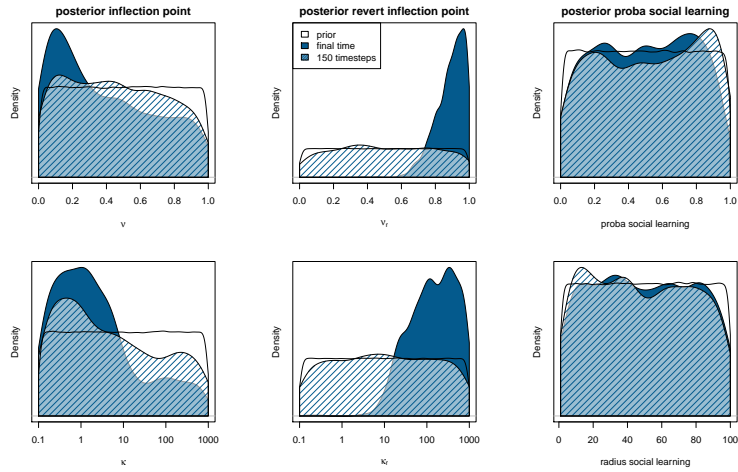
Figure S7: Same than figure 9 but for simulation run with variant D
