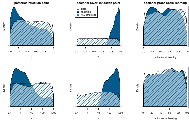
Figure S9: Same than figure 9 but for simulation run with variant F
