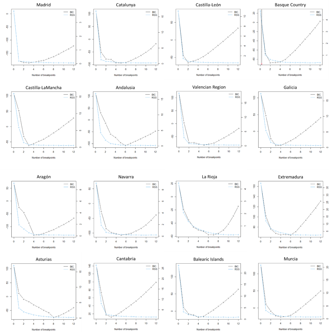
Figure S1: Goodness of fit of segmented regression models. RSS: residual sum of squares. BIC: bayesian information criterion.
