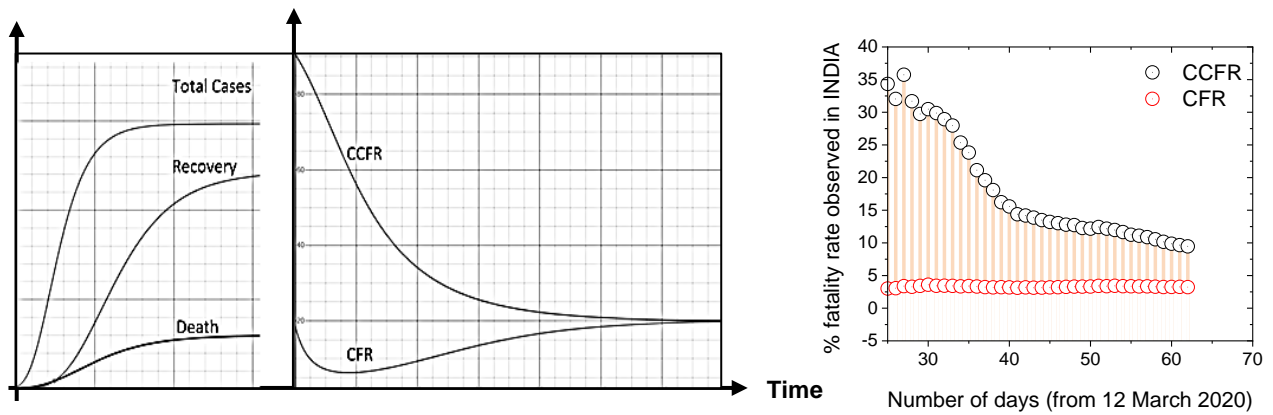
Figure S2: The dynamics of the fatality rates during a pandemic. LEFT: A simulated curve of CCFR and CFR using a modified SIR model (not discussed here) RIGHT: CCFR and CFR of INDIA calculated till 15 May 2020 (Data source: www.covid19india.org )
