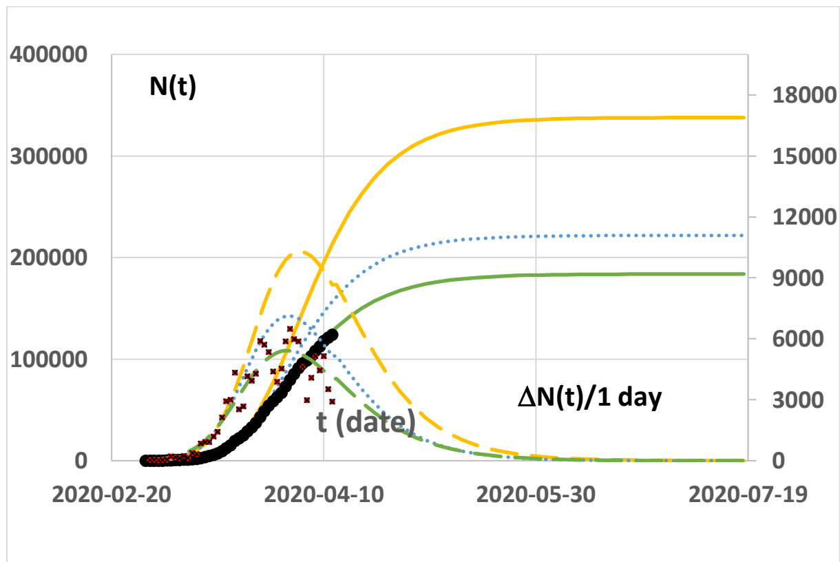
Figure 1: Linear plot of confirmed total number of infections in Germany as a function of time.
