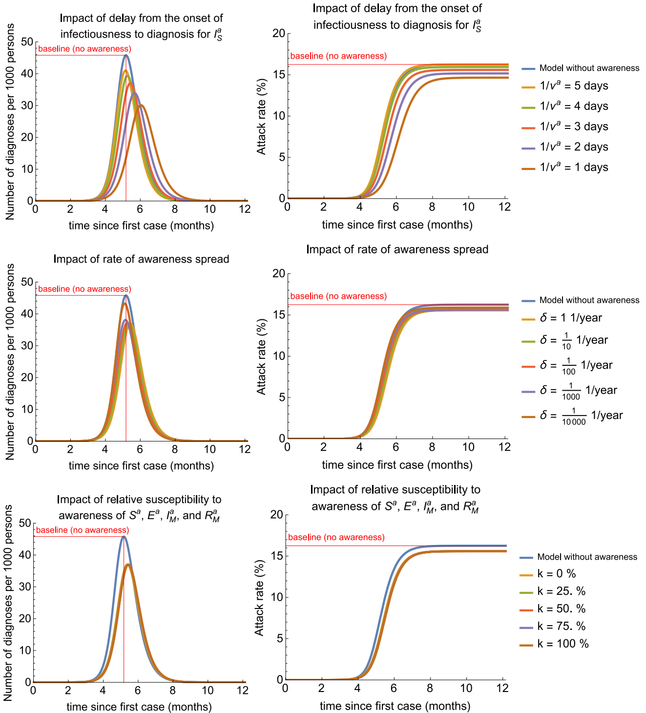
Figure 2. Sensitivity analyses of the transmission model with disease-awareness. Part 1.
