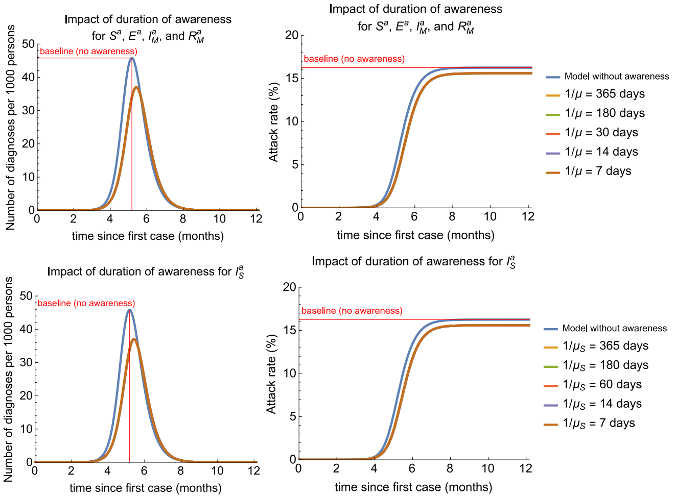
Figure 3. Sensitivity analyses of the transmission model with disease-awareness. Part 2.
