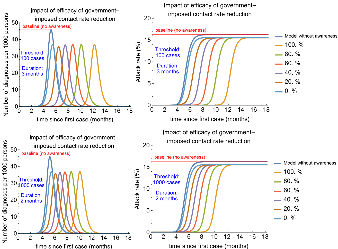
Figure 5. Sensitivity analyses of government-imposed social distancing intervention. Part 2.
