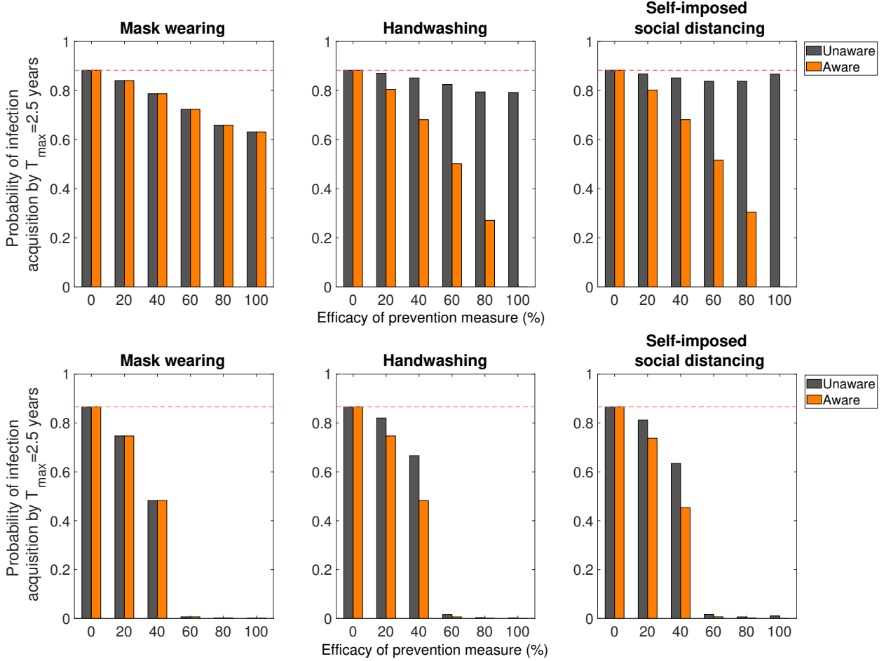
Figure 1. TOP figures were obtained for a slow rate of awareness spread. BOTTOM figures were obtained for a fast rate of awareness spread. The dashed red line indicates probability of infection in the model with awareness and no prevention measures.
