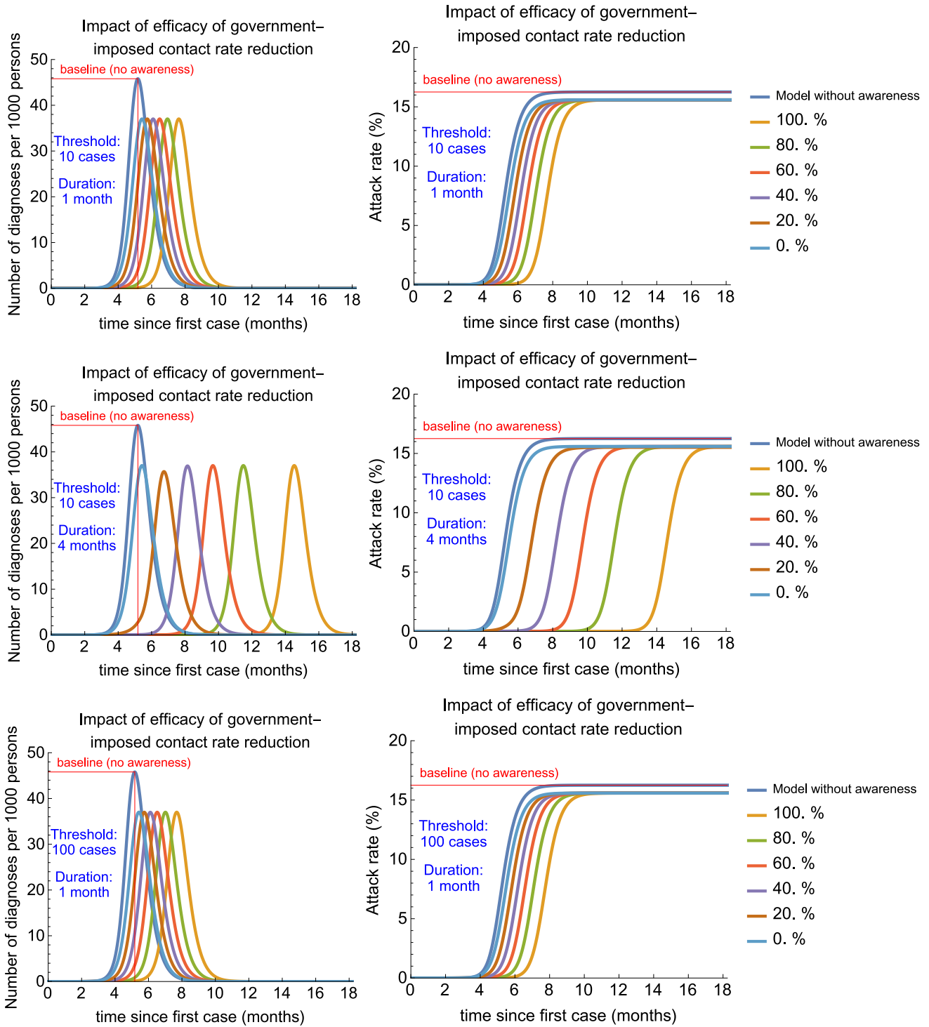
Figure 4. Sensitivity analyses of government-imposed social distancing intervention. Part 1.
