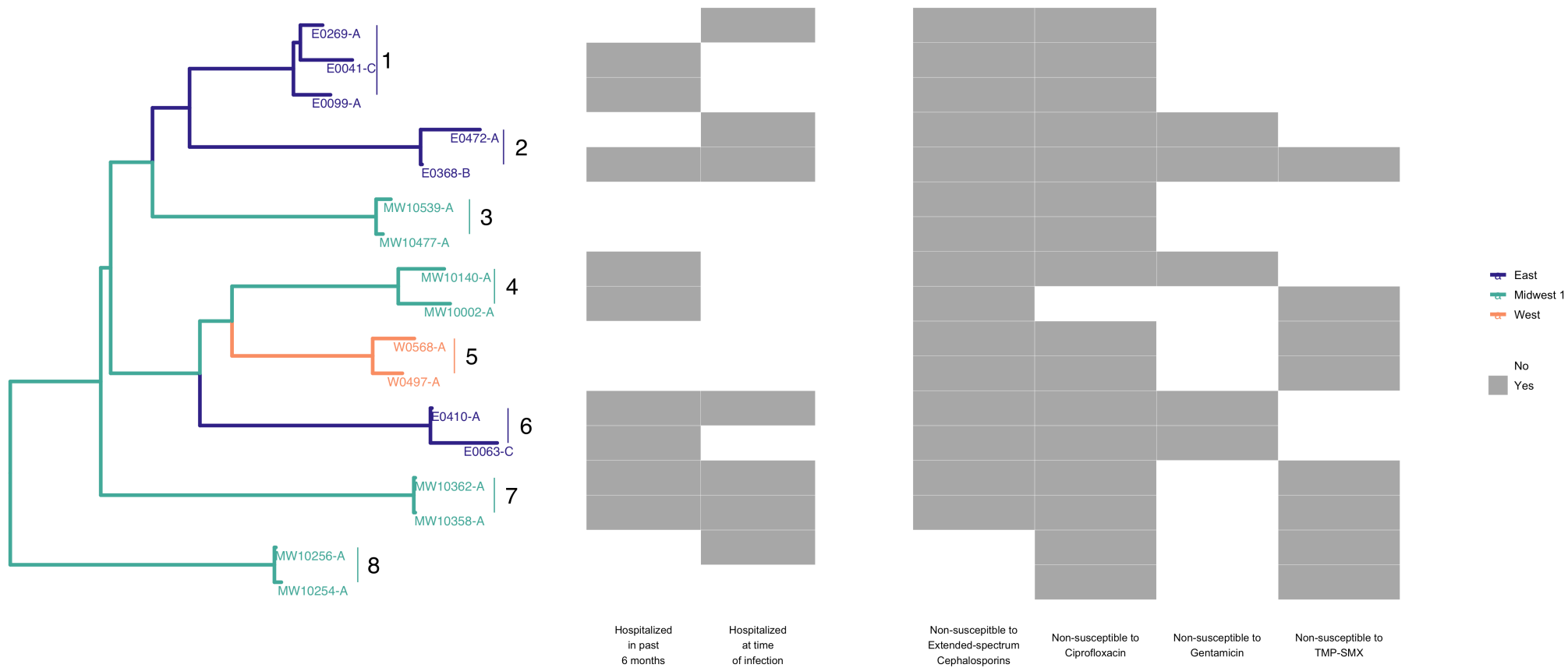
Supplementary Figure 2: Phylogeny of 8 identified putative transmission clusters colored by study site. Heatmap to the right of the phylogeny shows the presence or absence of selected patient characteristics and antibiotic susceptibilities.
