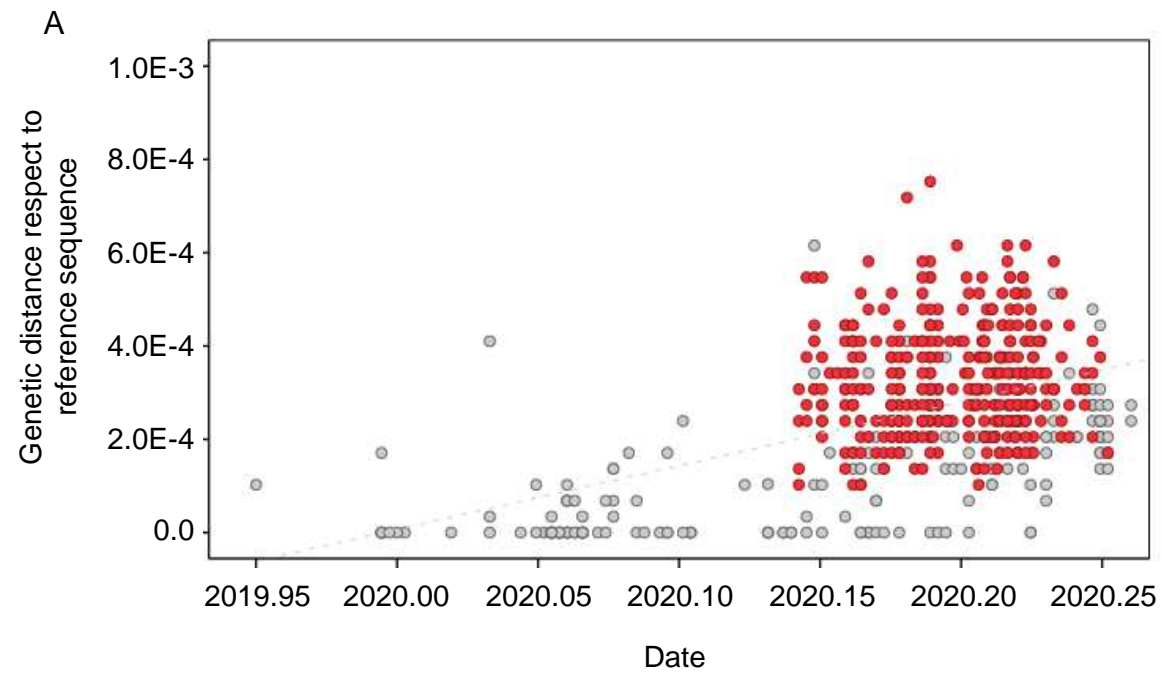
Supplementary Figure 3. (A) Genetic Distance for the Sars-Cov-2 Sequences against Collection Date. The Pearson correlation coefficient between genetic distance and collection date is displayed in the top-right corner ( r = 0.465 ). Sequences are colored by sampling location (North Italy= red, other location= gray) (B) Genetic Distance for the Sars-Cov-2 Sequences against lineages.
