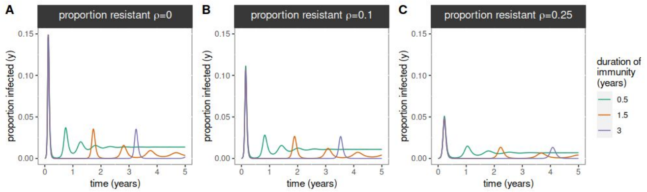
Figure S3 - Effect of duration of immunity. Time series of proportion infected ( y ) for varying proportion of resistant ( \rho ) and duration of immunity ( 1/\gamma , color scale) under proportionate mixing ( \delta = \rho ). Proportion of resistant ( \rho ) for each panel is presented on the title. Infectious period 1/\sigma = 5 days.
