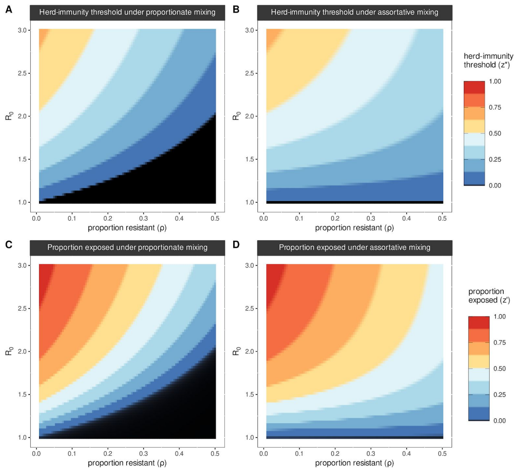
Figure S2 - Herd-immunity threshold and proportion exposed under proportionate and assortative mixing. Herd-immunity threshold ( z^* , panel A) when varying proportion of the population fully resistant ( \rho with R_{0_1} = 0 and R_0 = R_{0_2} ) under proportionate mixing ( \delta = \rho ). Panel B shows the same outputs but under assortative mixing ( \delta = 1 ). Proportion exposed ( z' , i.e. final exposed at the end of simulation) under proportionate mixing (C) and assortative mixing (D). Simulations ran for 365 days with an infectious period ( 1/\sigma ) of 5 days, \gamma = 0 . Each color band in the color scales equates to a 0.125 change, and black covers the range 0-0.01.
