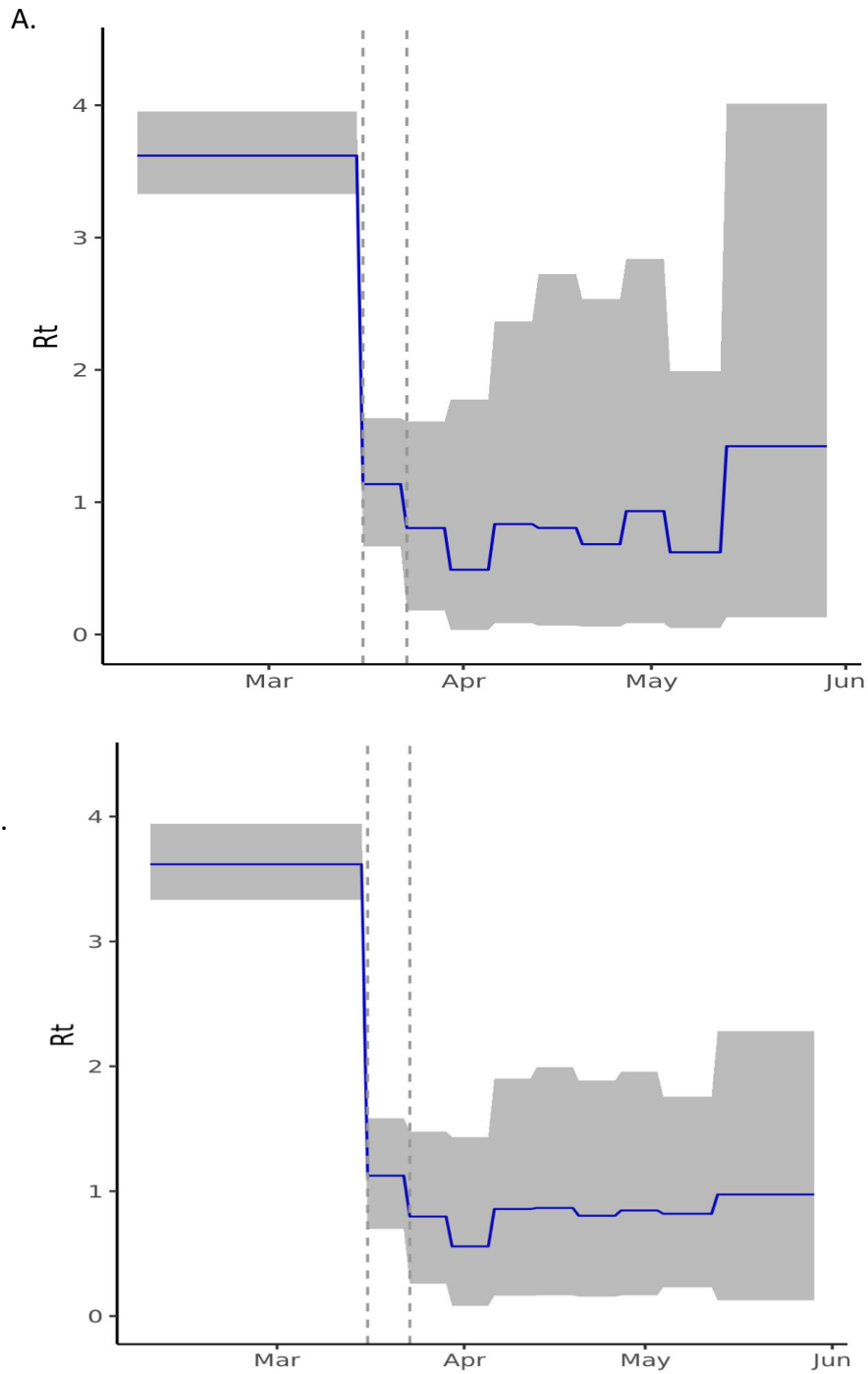
Supplementary Figure 3: R_t estimates with uninformative or broad priors
