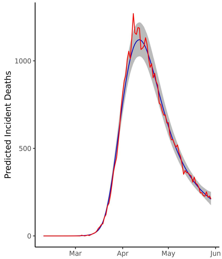
Supplementary Figure 5: Predicted and observed deaths in model with longer serial interval
