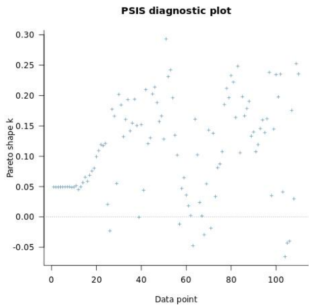
Supplementary Figure 2: Pareto shape parameter k distribution for final model
