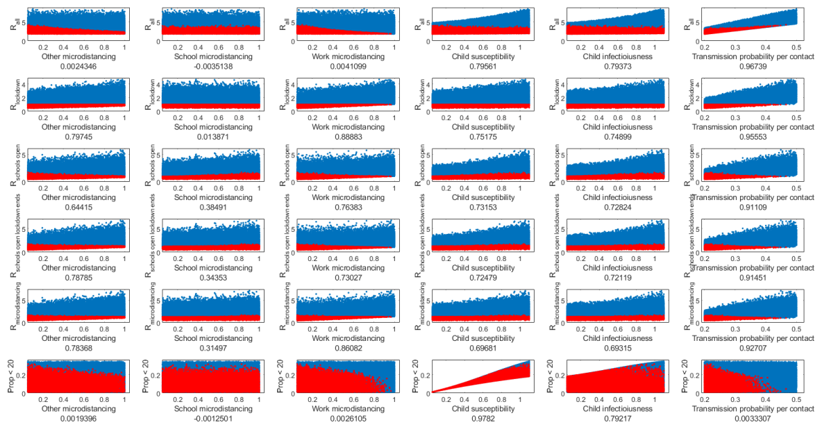
Figure 6. MCMC results using prior distributions for parameters given in Table 3 above. The values for which the R_{eff} is <1 for the full lockdown are shown in red. The partial correlation is provided for each parameter/outcome pair.
