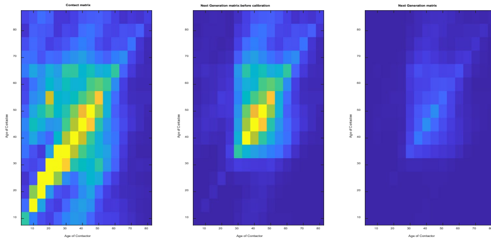
Figure 2. A comparison between the contact matrix and the next generation matrix for China. Left panel is the contact matrix for China taken from Prem et al. 1 Middle column is the matrix following changes made to relative infectiousness and relative susceptibility by age. Right panel is the final calibrated next generation matrix for China of 2.684.
