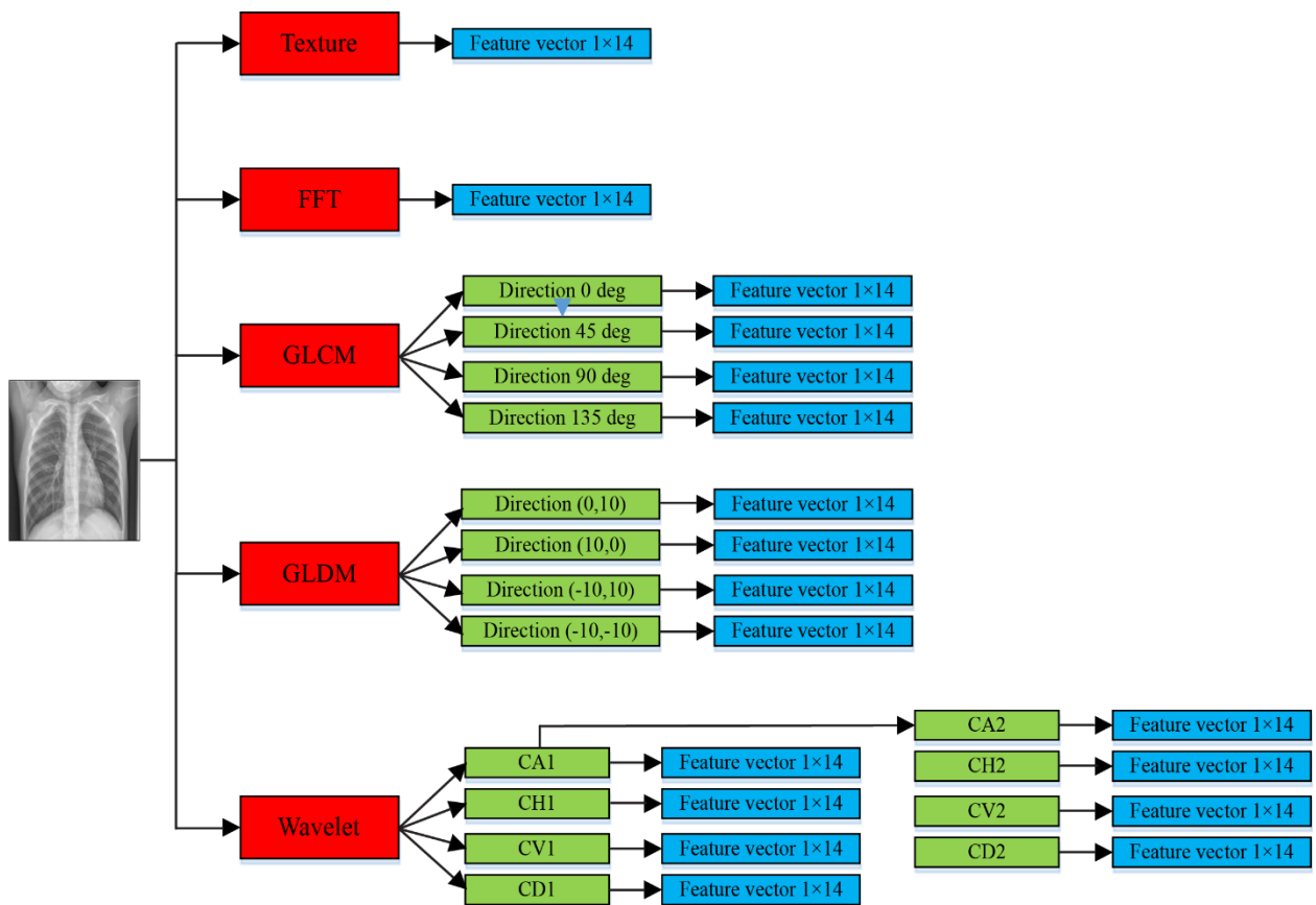
Supplementary Figure 1: The proposed feature extraction schematic diagram
