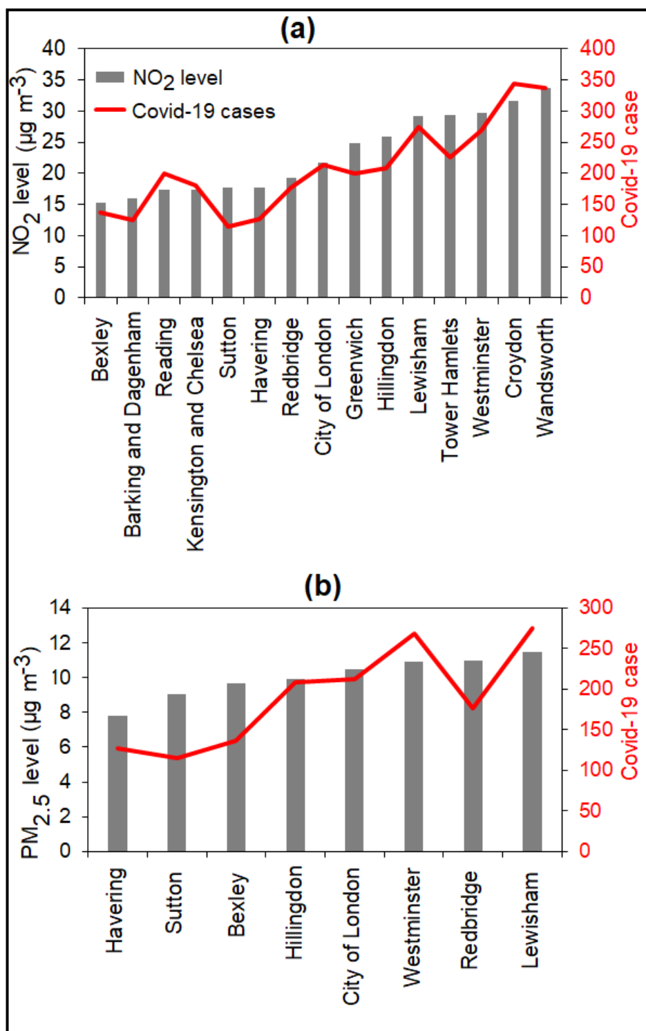
Figure S1. Relationship between average a) NO 2 and b) PM 2.5 pollution concentrations and reported COVID-19 cases for different boroughs in London for March 2020. The grey bars show the monthly average of NO 2 and PM 2.5 concentrations and the line represent the cumulative number of reported COVID-19 cases in each London borough.
