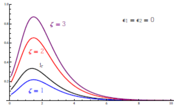
165 Figure A.5: Real population of infectives versus three 166 different measured values of the infective population in 167 Hypothetical Scenario 1, where \varepsilon_1 = \varepsilon_2 = 0 .
