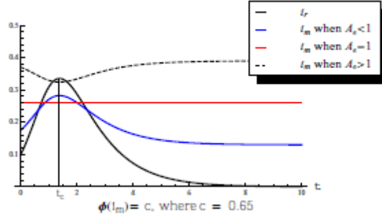
178 Figure A.6: Example of Response to Hypothetical
