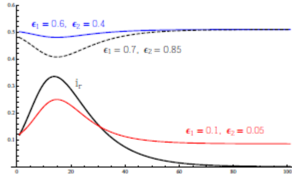
336 337 Figure A.11: Examples of Scenario 1-type disease with j 338 non-constant: Graphs of i_m for different \varepsilon 's with 339 p=q=10 340
