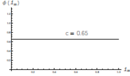
117 Figure 4: \phi(i_m) = c , where c is a constant and 0 < c \leq 1 .
