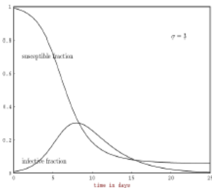
Figure 2: Time in days
