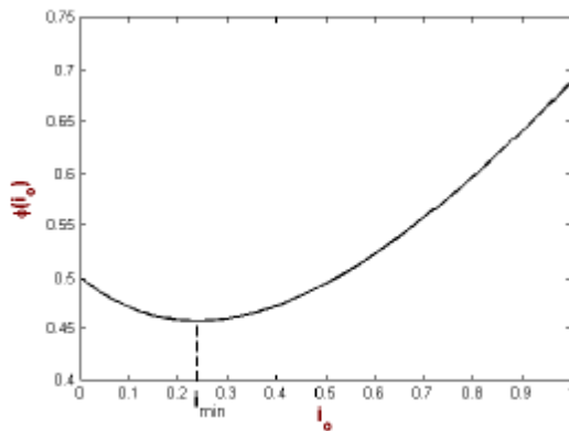
Figure 7: \phi(i_m) = k(e^{-bi_m} + ci_m) where 0 < k < 1 .
