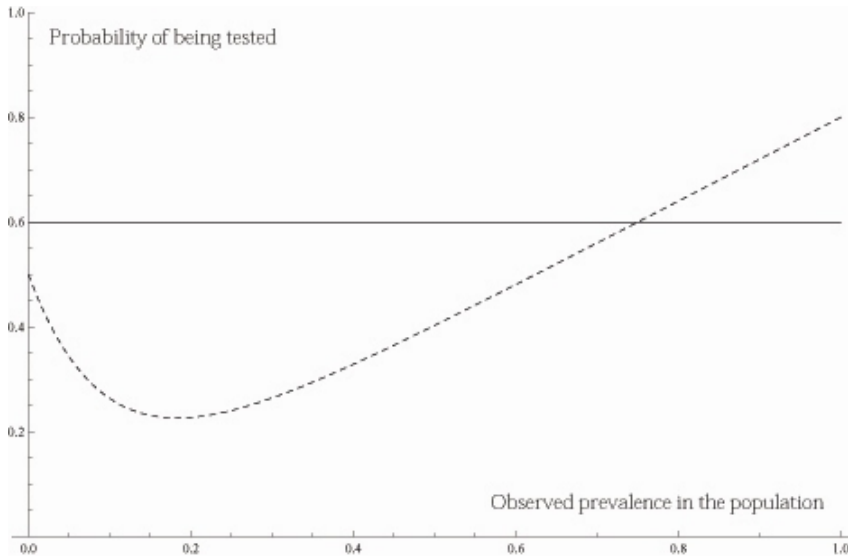
79 80 Figure A.3. The two hypothetical \phi functions used for demonstration; defined in Table 81 A.2.
