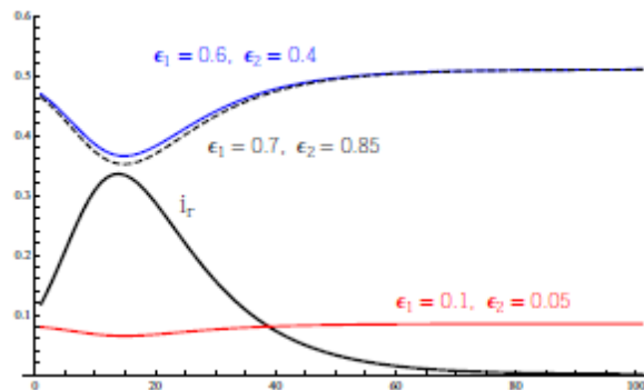
Figure A.12: Examples of Scenario 1-type disease with j
