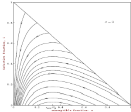
Figure 1: Phase portrait of S-I-R model
