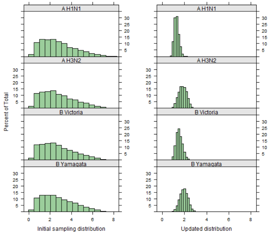
Figure S2.2: Distributions of basic reproductive number R_0 : 7,198 samples without fit criteria applied (left), and the 7,198 runs of the calibrated model (right).
