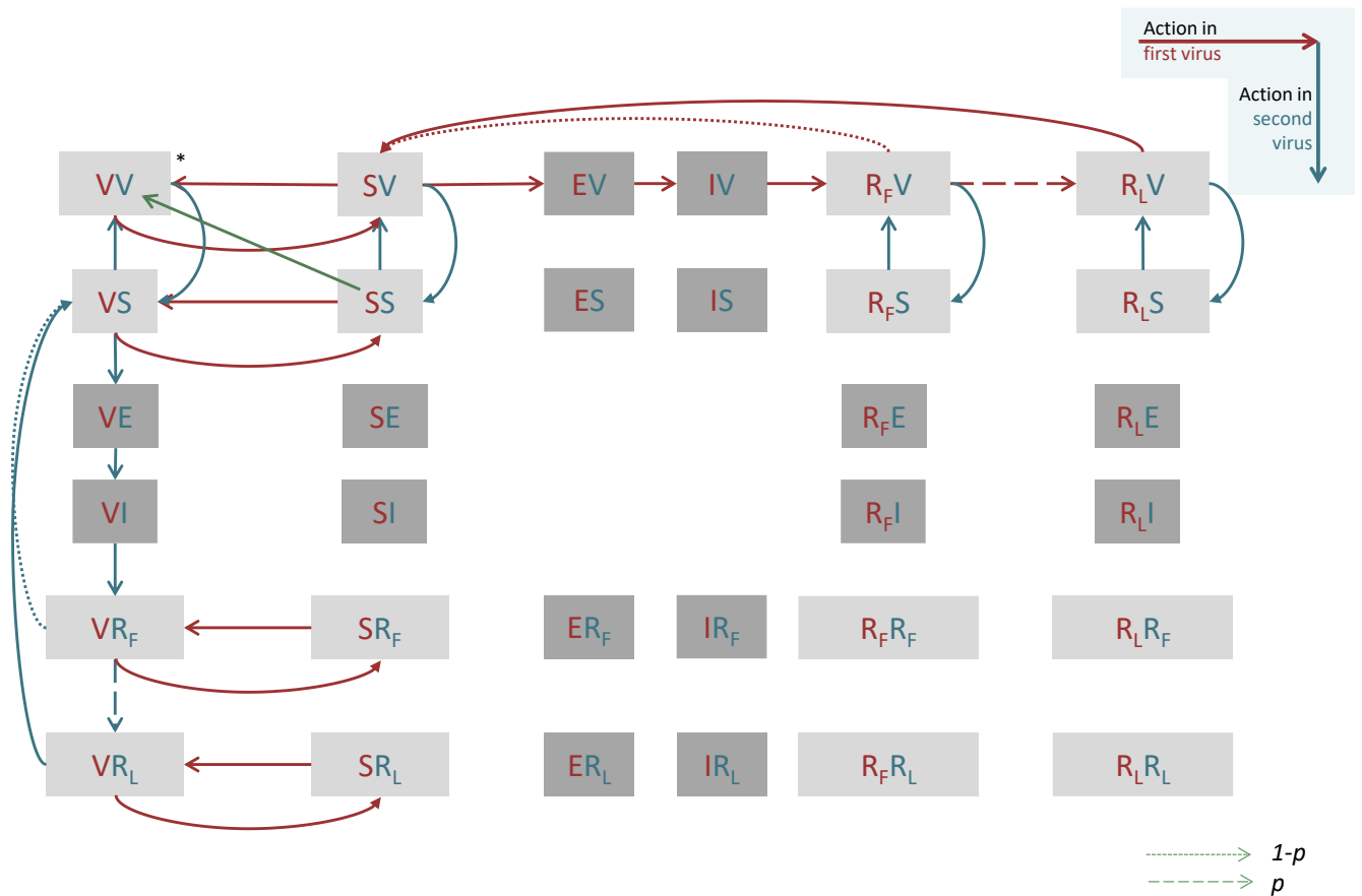
Figure S1.3: Combined model structure including vaccination. Details of model flows between compartments with no vaccinated individuals are left out for simplicity as they are detailed in Figure S1.2.
