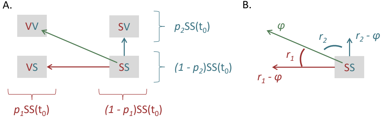
Figure S1.5: The proportion of the original susceptible population vaccinated to each virus at time t_0 + \Delta t_v , given an originally unvaccinated population.
