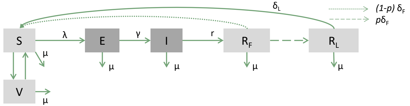
Figure S1.1: Conceptual transmission model structure for a single virus. This diagram does not represent the full model, in which two influenza strains were modelled simultaneously. Flow parameters are explained in Table S1.2.
