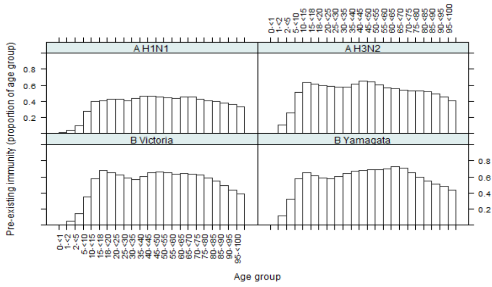
Figure S1.4: Pre-existing immunity structure.
