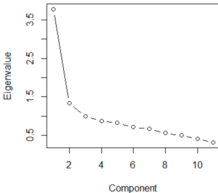
Supplementary Figure S3. Scree plot of eigenvalues from 11 UK Biobank cognitive tests
