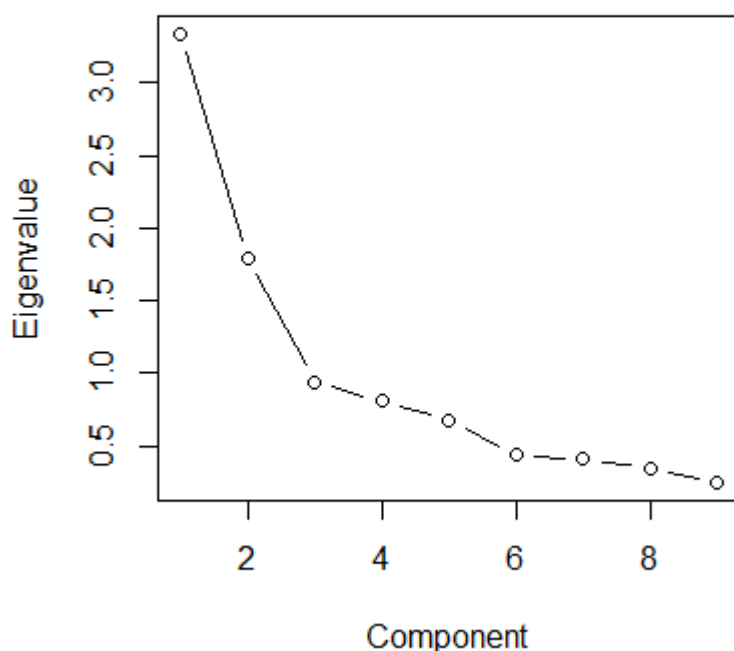
Supplementary Figure S5. Scree plot of eigenvalues from 9 reference cognitive tests (excluding reference tests with overlapping items with the UK Biobank tests)
