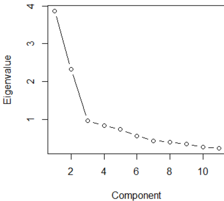
Supplementary Figure S2. Scree plot of eigenvalues from 11 reference cognitive tests
