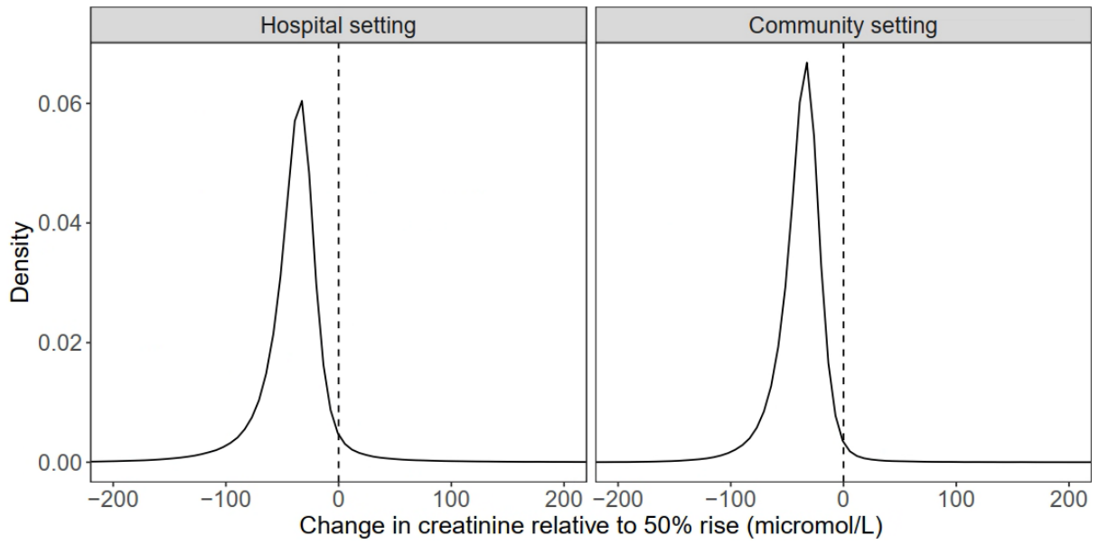
Fig S4. Distribution of the centred running variable for the hospital and community setting.
