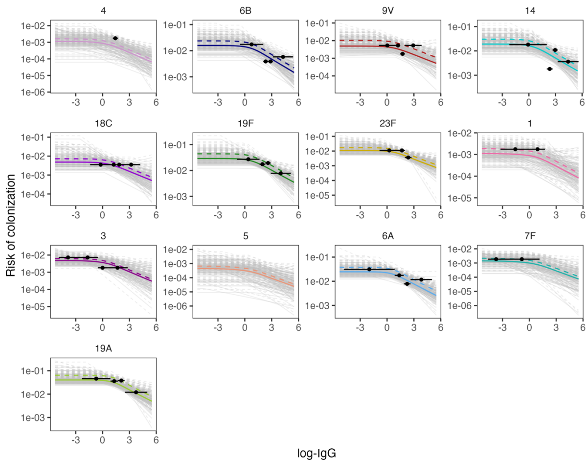
eFigure 5. The observed proportion of colonization and predicted risk of colonization by antibody concentration for each serotype
