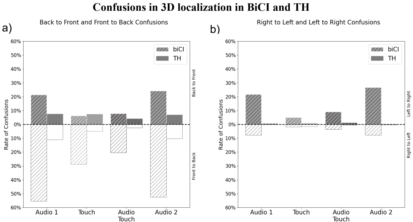
Figure 4. Front-Back and Right-Left confusions as percentage, in the typically hearing and in users of bilateral cochlear implants.
