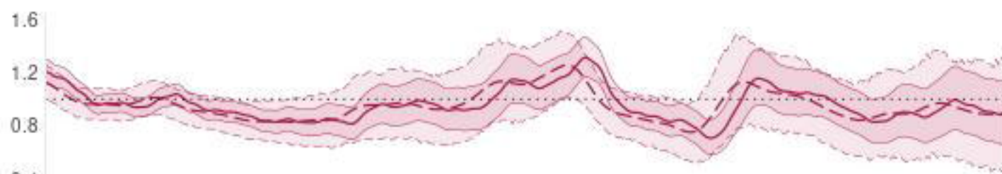
(D) STEP 3: Produce county-level R_e via population weighting
