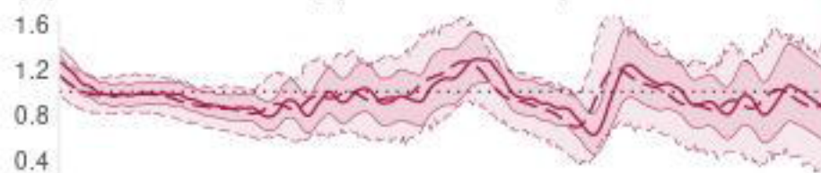
(C) STEP 2: Produce R_e (sewershed-level)
