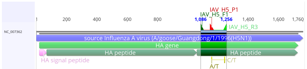
Figure S1. Location of the primers and probe within a reference genome (NC_007362). Within the HA segment of A/goose/Guangdong/1/1996 , ( https://www.ncbi.nlm.nih.gov/datasets/taxonomy/93838/ ), the amplicon is located between bases 1086-1256. IAV_H5_P1 is the probe, IAV_H5_F1 and IAV_H5_R3 are the forward and reverse primers, respectively.
