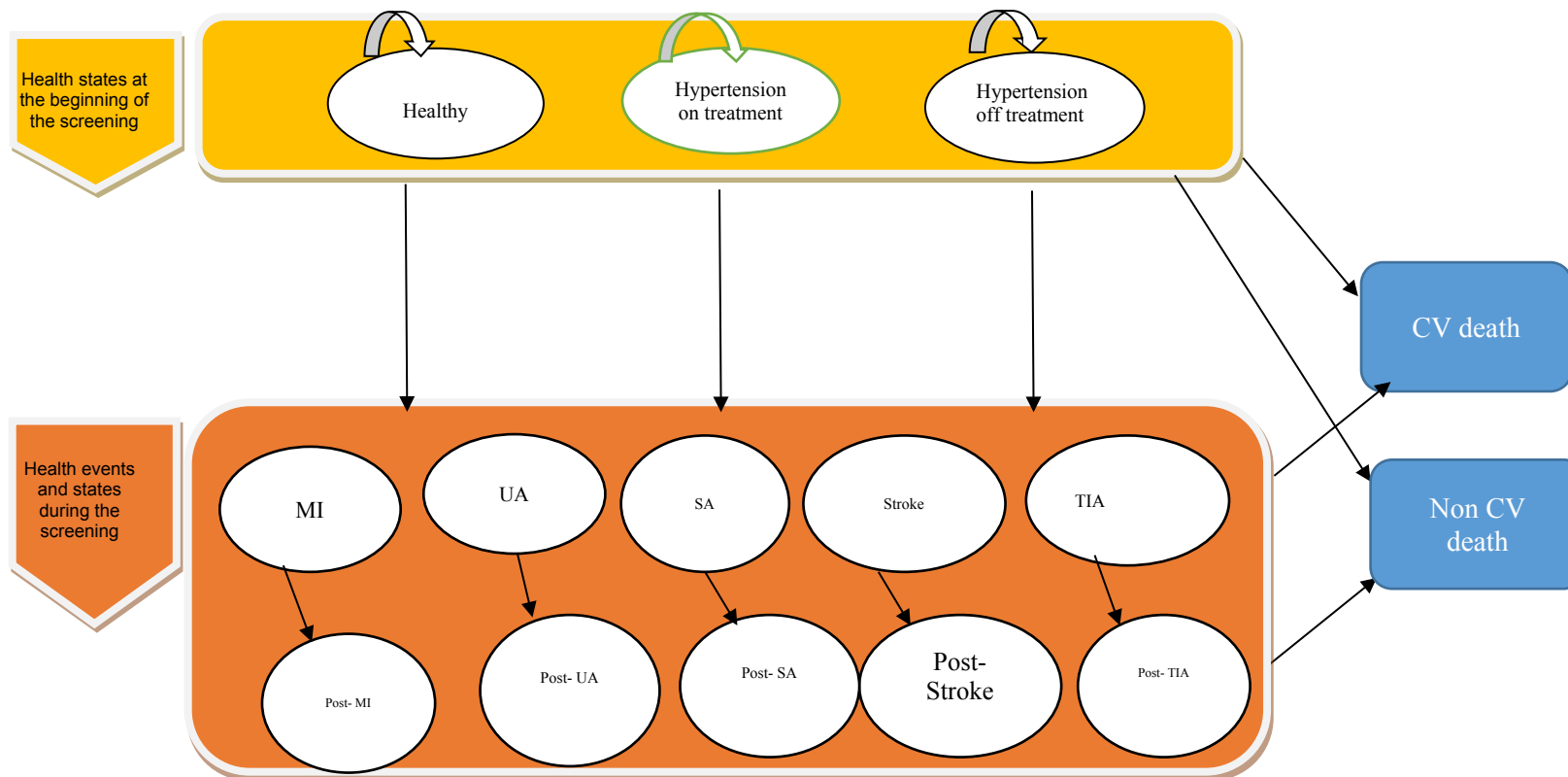
Figure 1: Markov model structure
