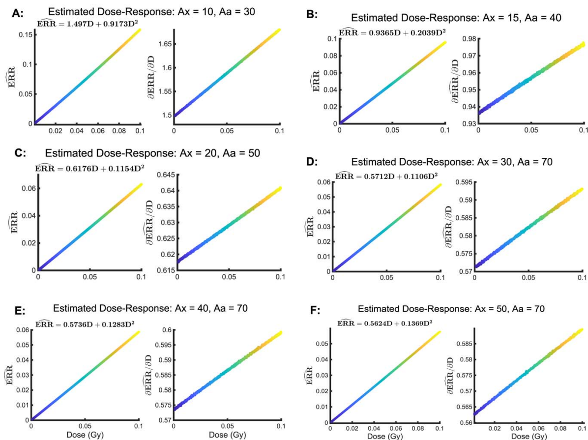
Figure 4: Estimated Excess Relative Risk (ERR) and its first-order partial derivative for different ages at exposure ( A_x ) and attained ages ( A_a ) for a woman residing in Nagasaki. A: A_x = 10 and A_a = 30 ; B: A_x = 15 and A_a = 40 ; C: A_x = 20 and A_a = 50 ; D: A_x = 30 and A_a = 70 ; E: A_x = 40 and A_a = 70 ; F: A_x = 50 and A_a = 70 .
