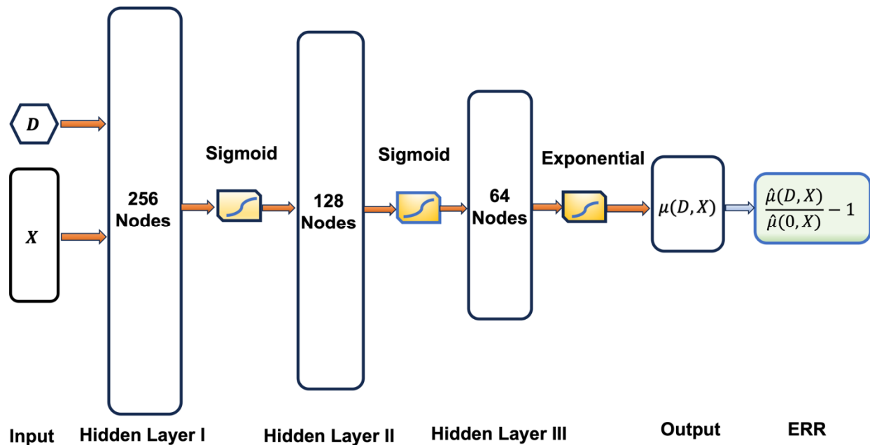
Figure 1: Neural network structure for radiation risk prediction, where D and X represent the radiation dose and confounding factors, respectively. ERR stands for excess relative risk. The architecture includes 3 hidden layers with node counts of 256, 128, and 64, respectively. Both sigmoid and exponential activation functions were employed. The estimation of ERR is indicated in the rightmost shaded box, determined after model training.
