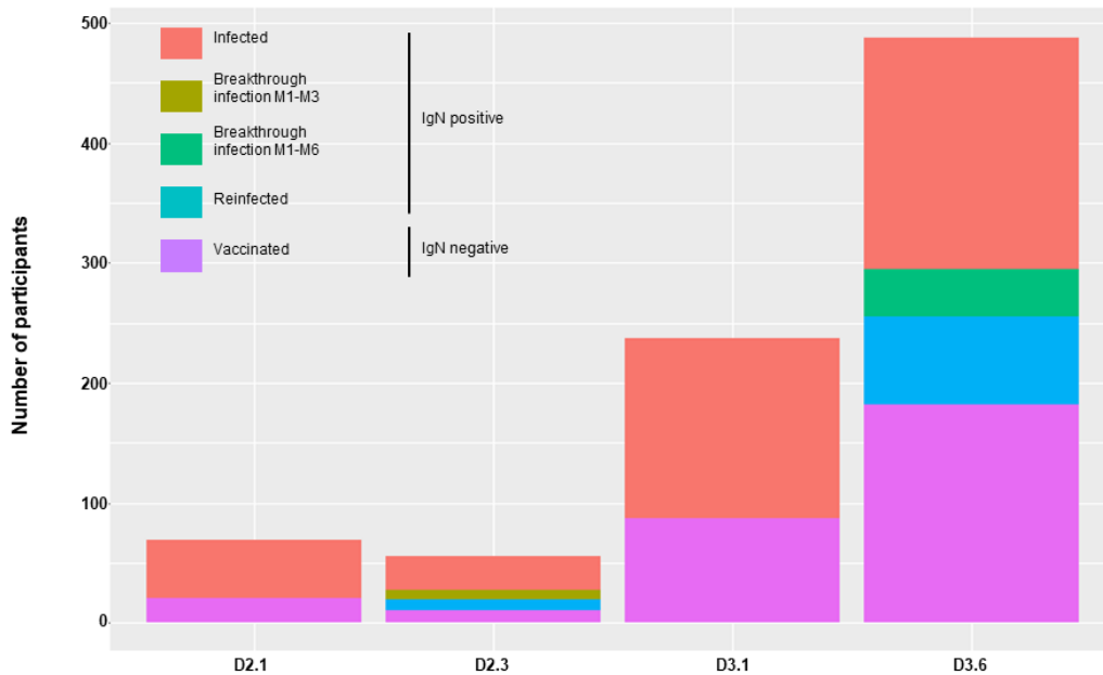
Distribution of the 849 samples
