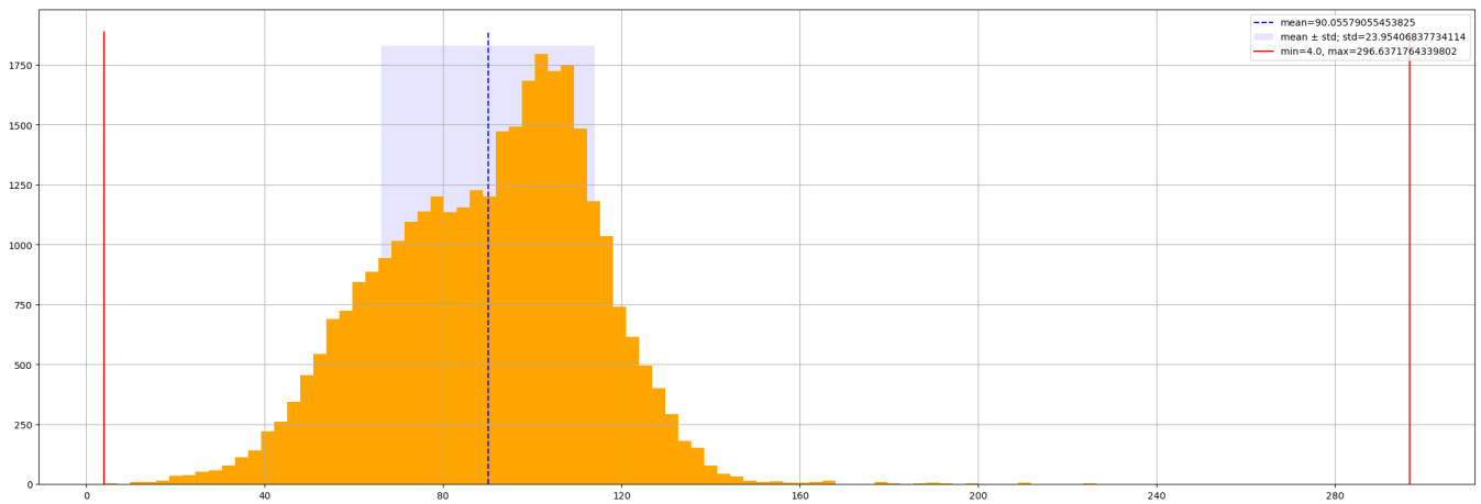
Figure 12: Feature distribution: degfr_base.
