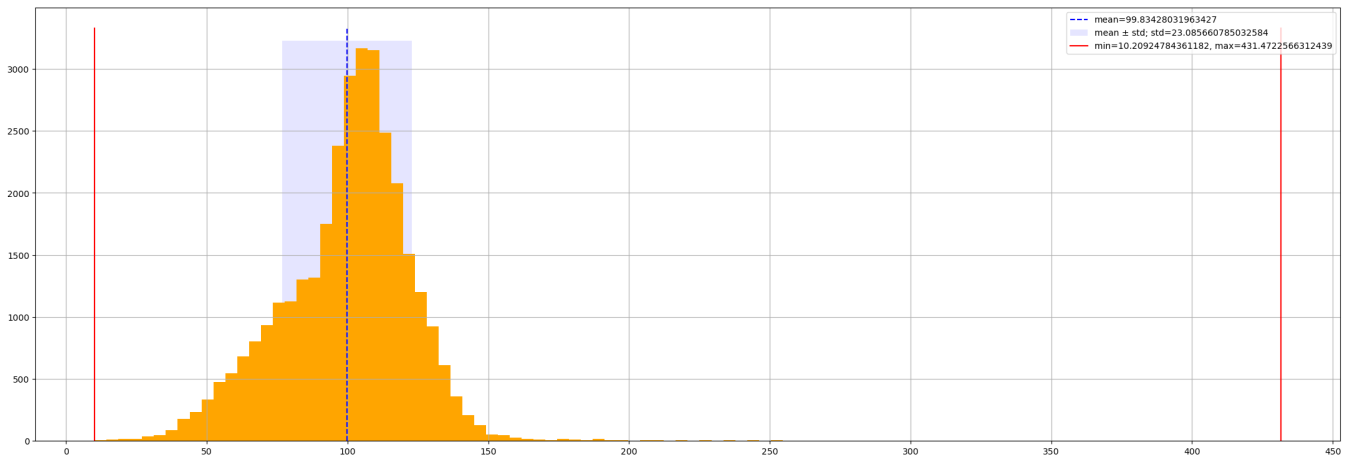
Figure 13: Feature distribution: degfr_max.
