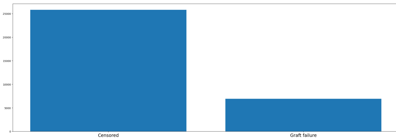
Figure 37: Target distribution: gcens.
