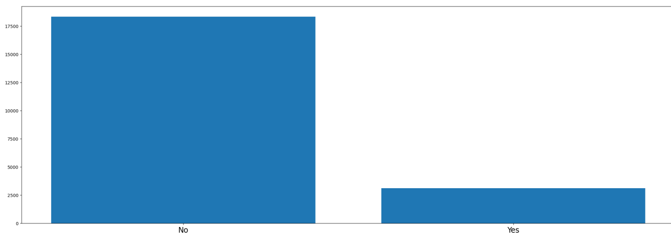
Figure 16: Feature distribution: dpast_alcohol_abuse.
