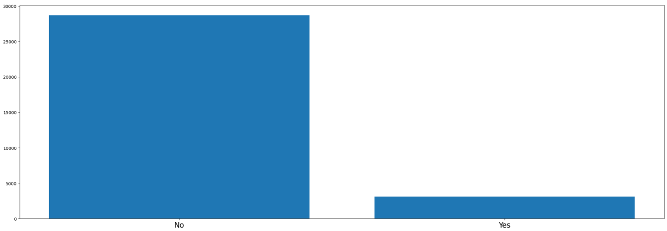
Figure 17: Feature distribution: dpast_cardio_disease.
