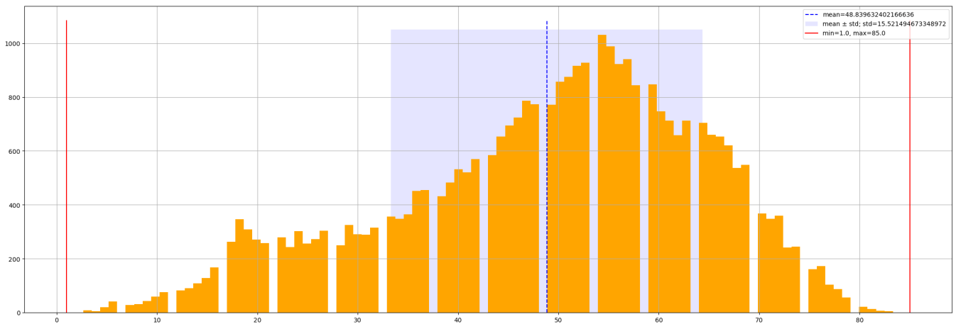
Figure 8: Feature distribution: dage.
