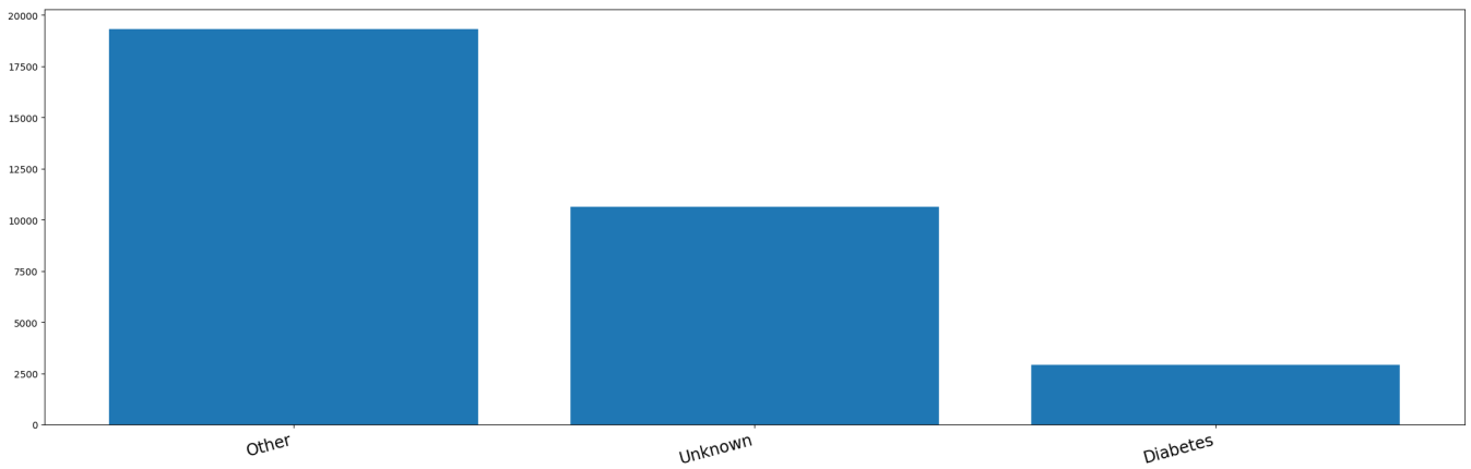
Figure 28: Feature distribution: prd.
