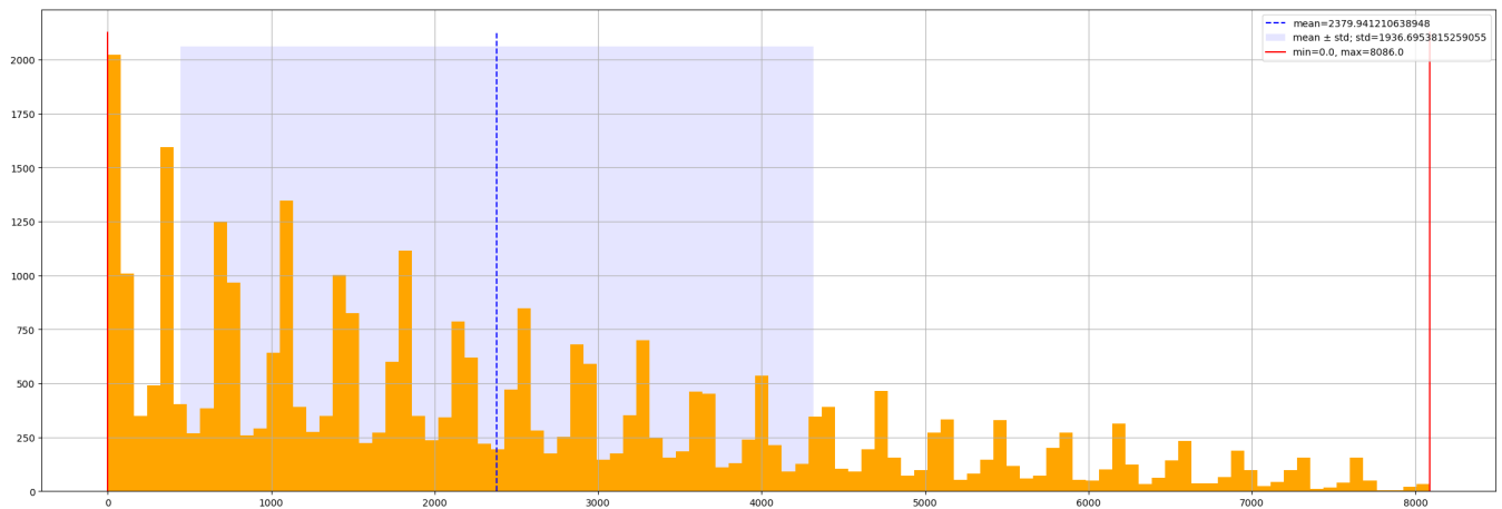
Figure 38: Target distribution: gsurv.
