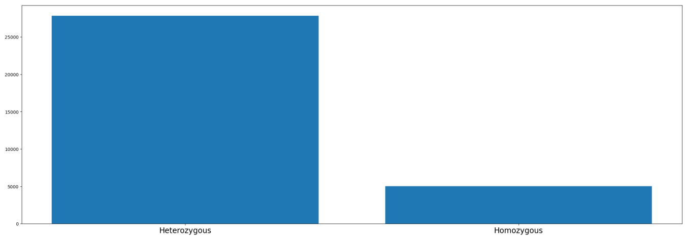
Figure 29: Feature distribution: r_dr_hom.
