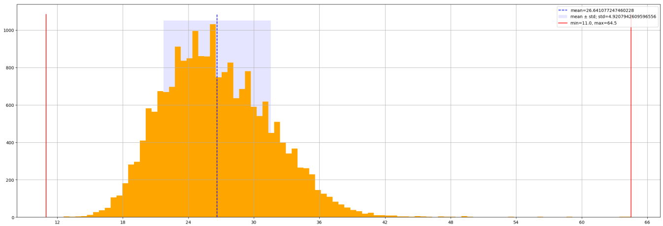
Figure 32: Feature distribution: rbmi.
