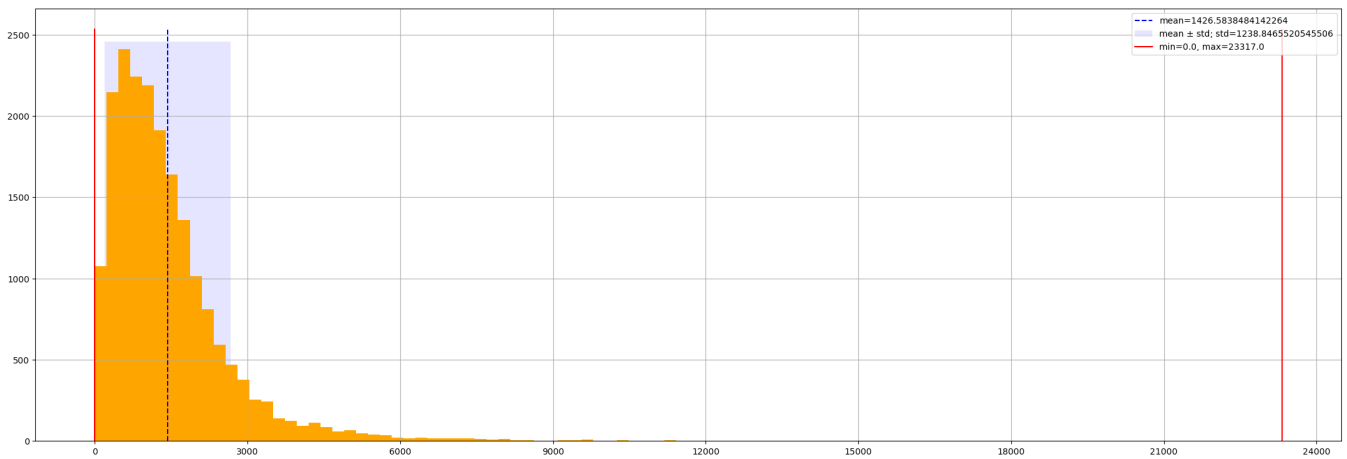
Figure 14: Feature distribution: dial_days.
