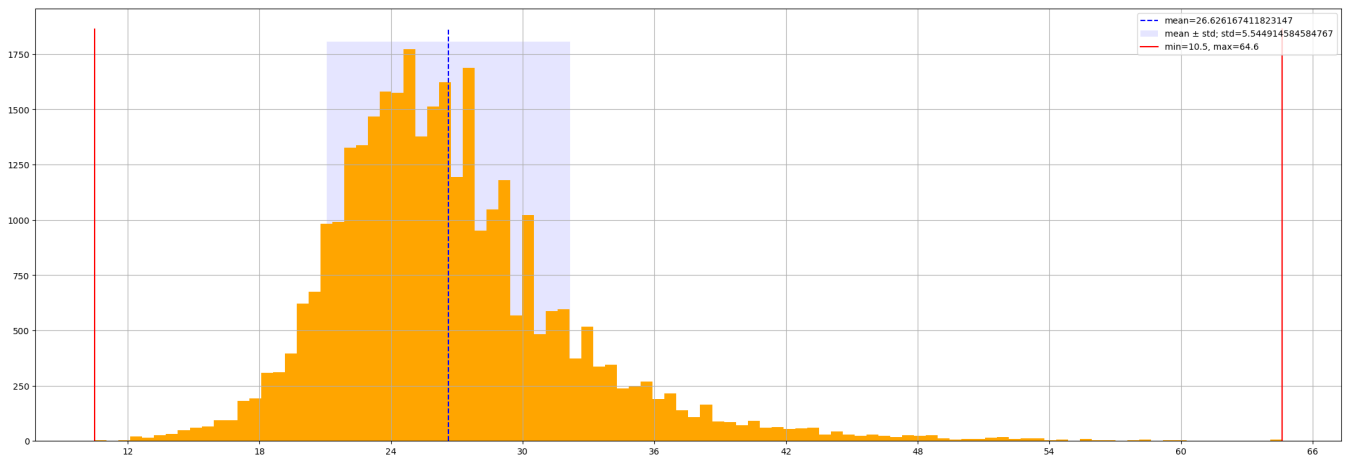
Figure 9: Feature distribution: dbmi.
