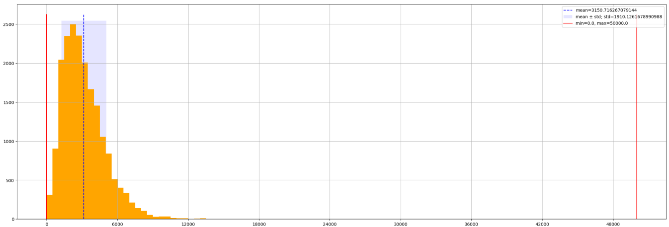
Figure 24: Feature distribution: durine_output_24hrs.
