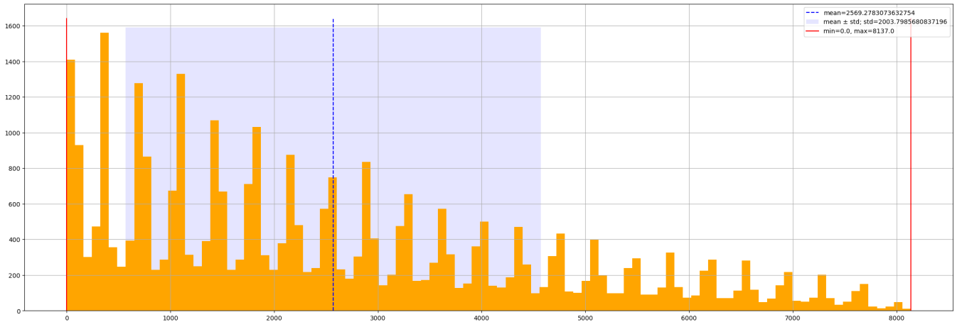
Figure 40: Target distribution: psurv.
