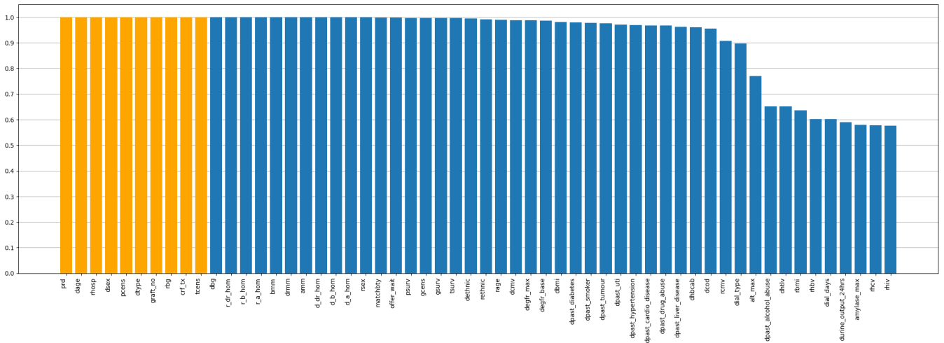
Figure 1: Features densities. A density of 1 means that the corresponding feature is always present; conversely, a density of 0 means that this feature is always missing. Orange columns highlight features with no missing value at all.
