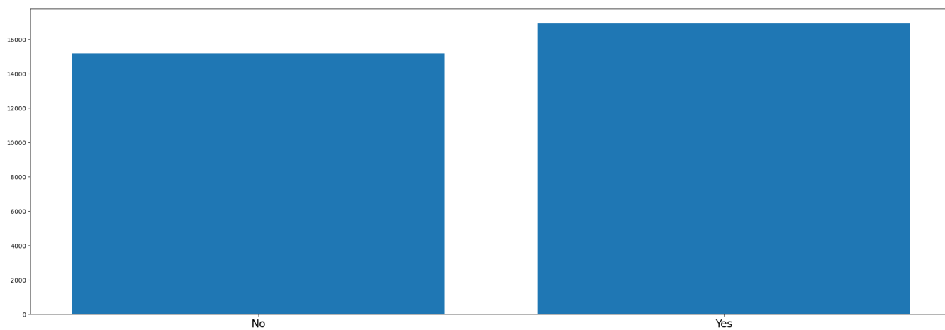
Figure 20: Feature distribution: dpast_smoker.
