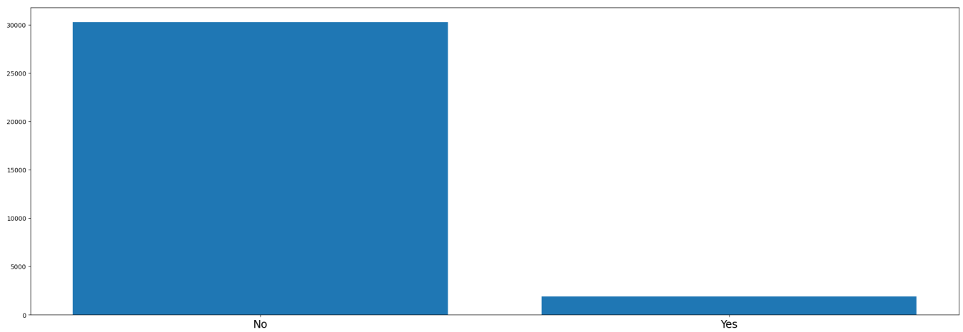
Figure 18: Feature distribution: dpast_diabetes.
