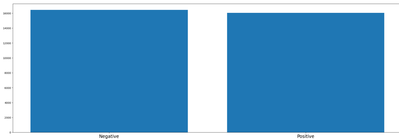
Figure 10: Feature distribution: dcmv.
