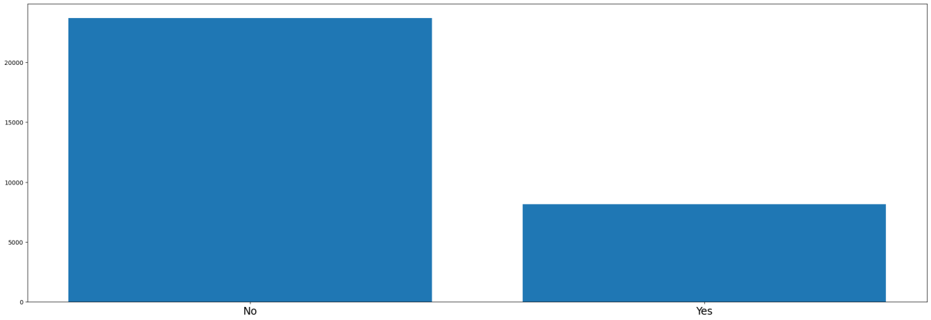
Figure 19: Feature distribution: dpast_hypertension.
