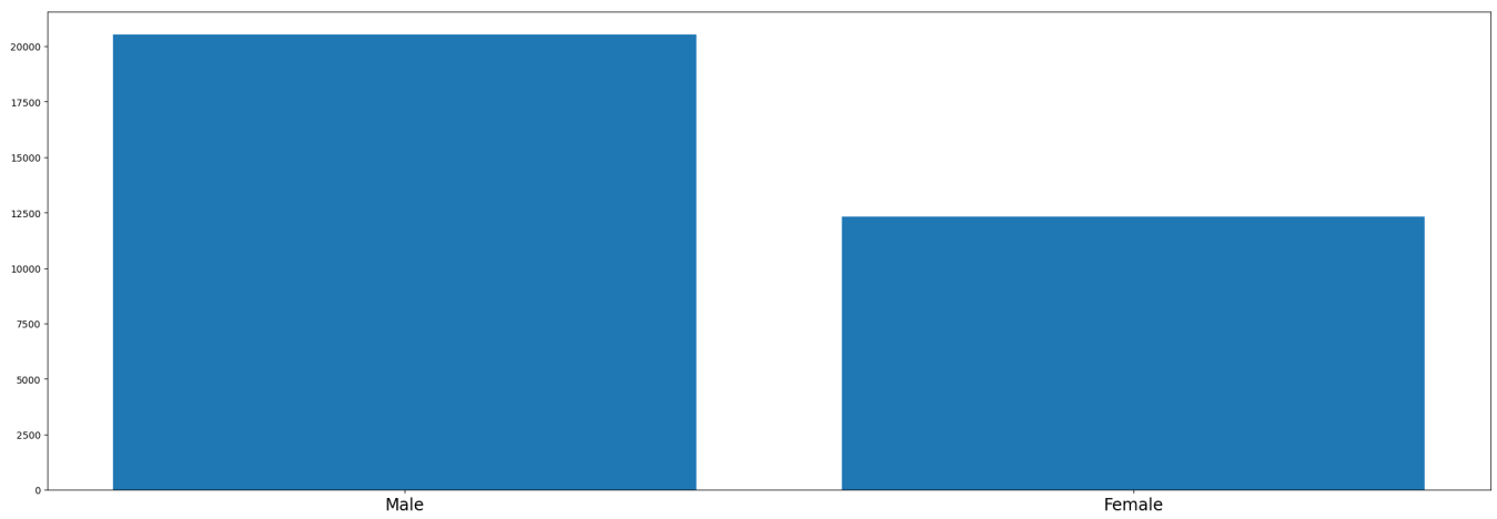
Figure 36: Feature distribution: rsex.
