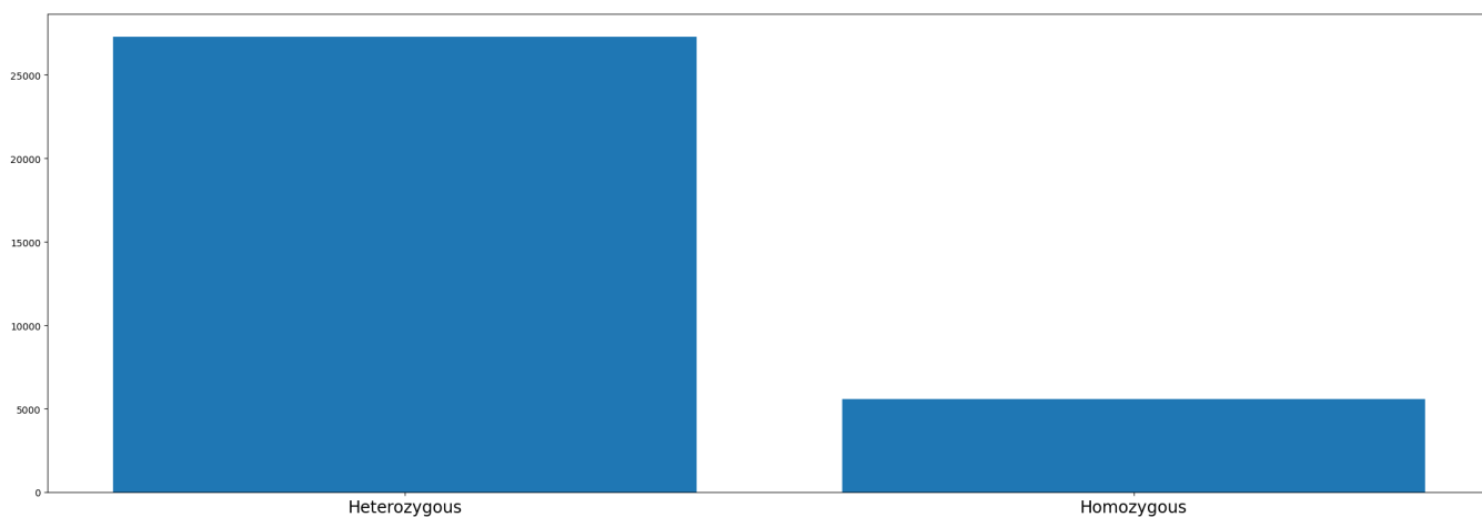
Figure 5: Feature distribution: d_a_hom.
