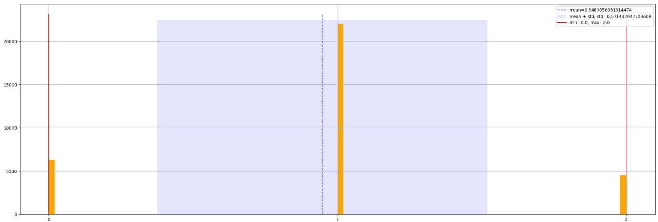
Figure 3: Feature distribution: bmm.
