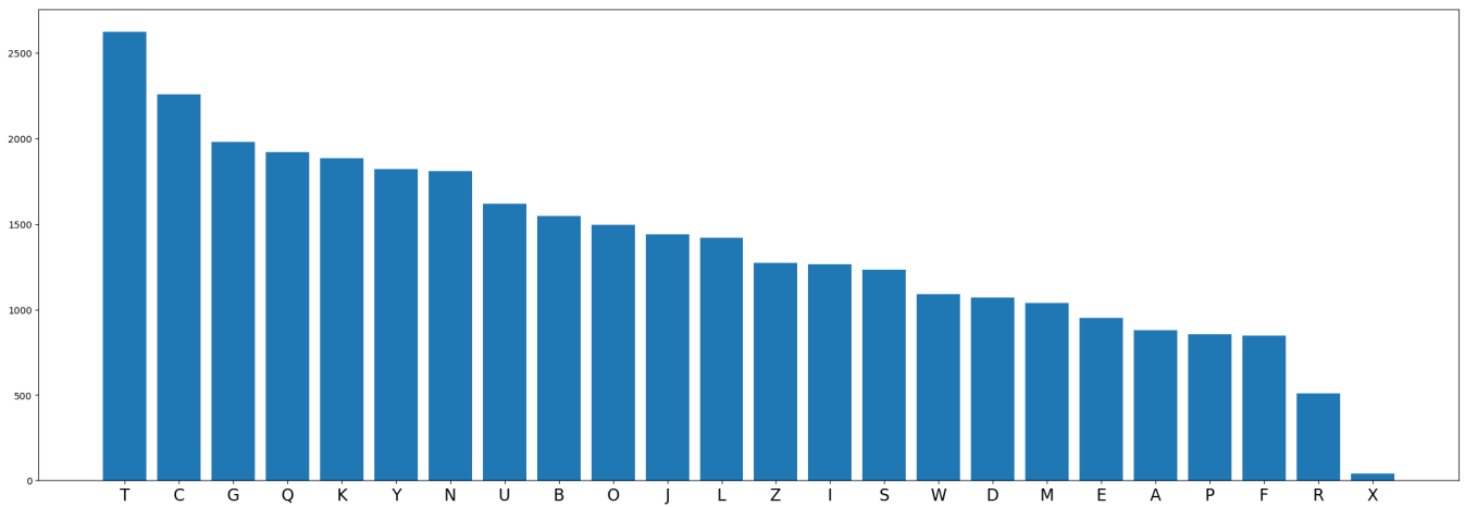
Figure 35: Feature distribution: rhosp.
