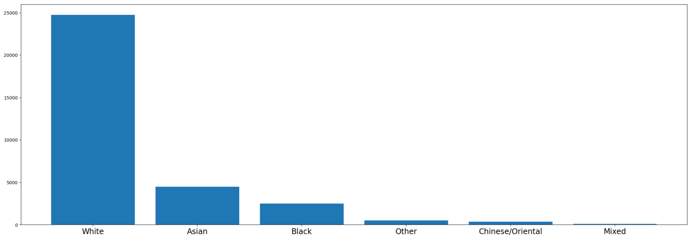
Figure 34: Feature distribution: rethnic.
