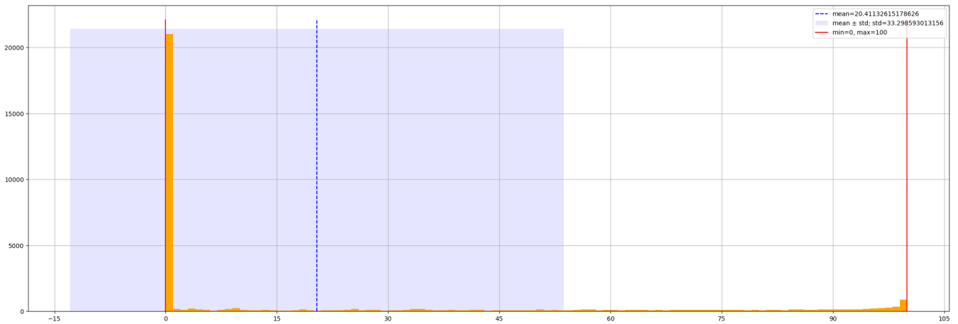
Figure 4: Feature distribution: crf_tx.
