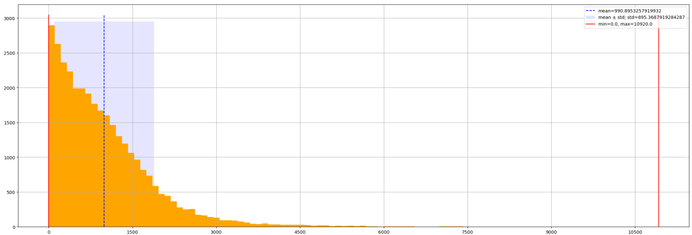
Figure 27: Feature distribution: offer_wait.
