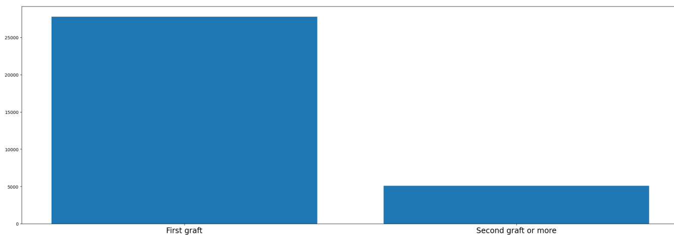
Figure 25: Feature distribution: graft_no.
