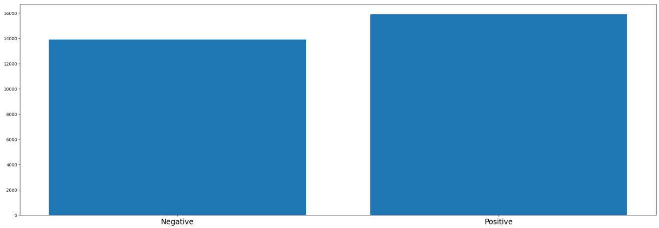
Figure 33: Feature distribution: rcmv.
