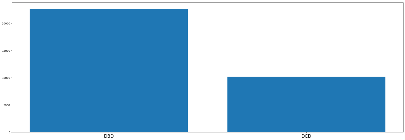
Figure 23: Feature distribution: dtype.
