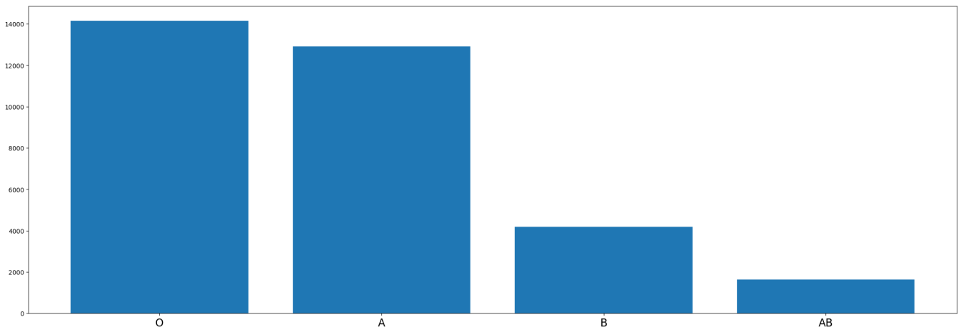
Figure 31: Feature distribution: rbg.
