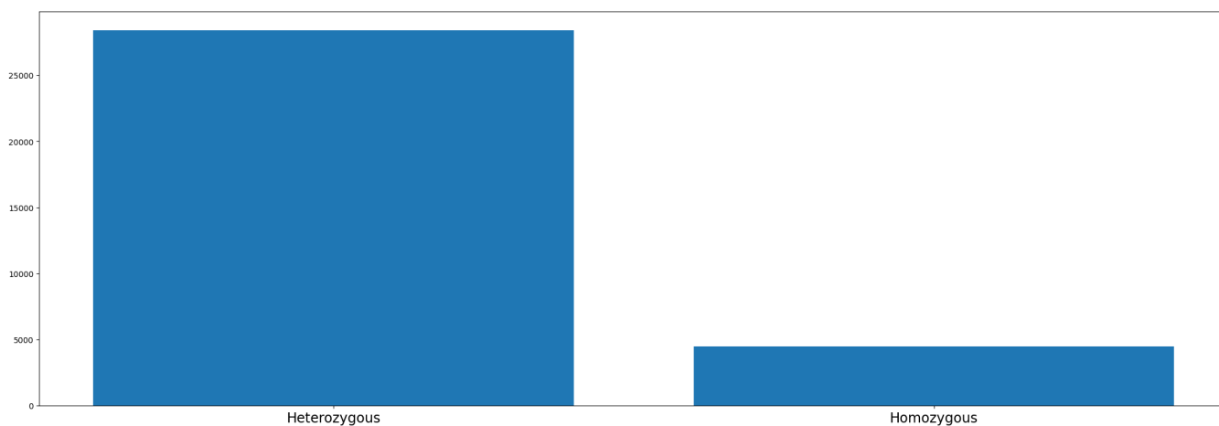
Figure 7: Feature distribution: d_dr_hom.
