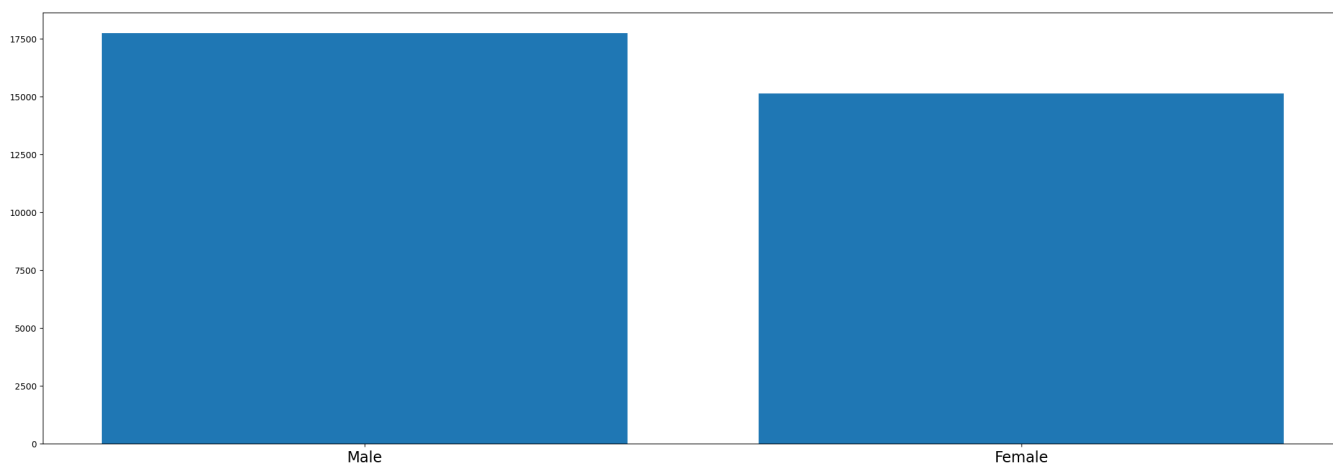
Figure 22: Feature distribution: dsex.
