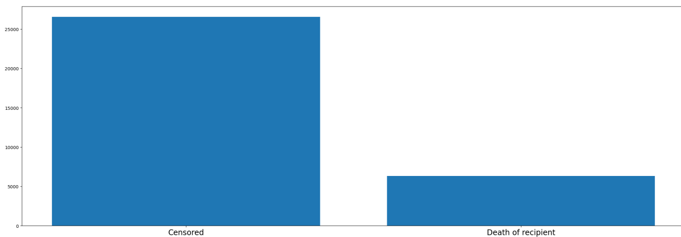
Figure 39: Target distribution: pcens.
