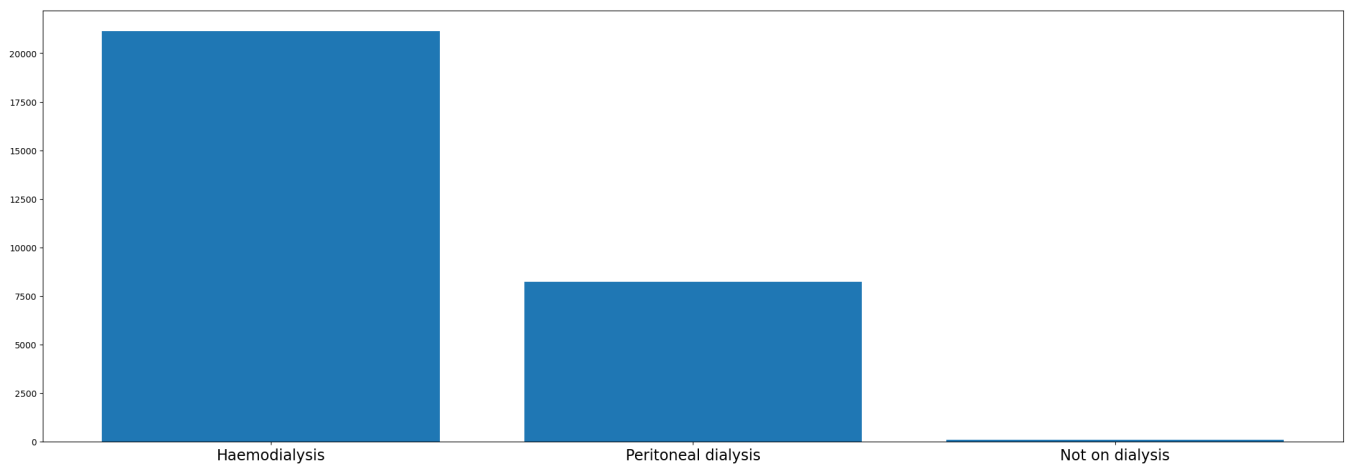
Figure 15: Feature distribution: dial_type.
