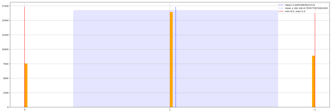
Figure 2: Feature distribution: amm.
