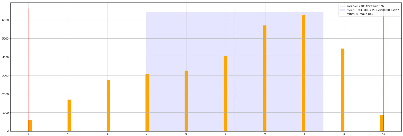
Figure 26: Feature distribution: matchbty.
