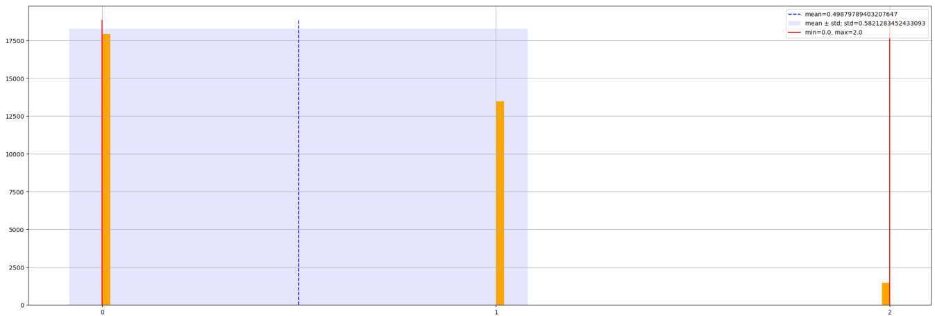
Figure 21: Feature distribution: drmm.
