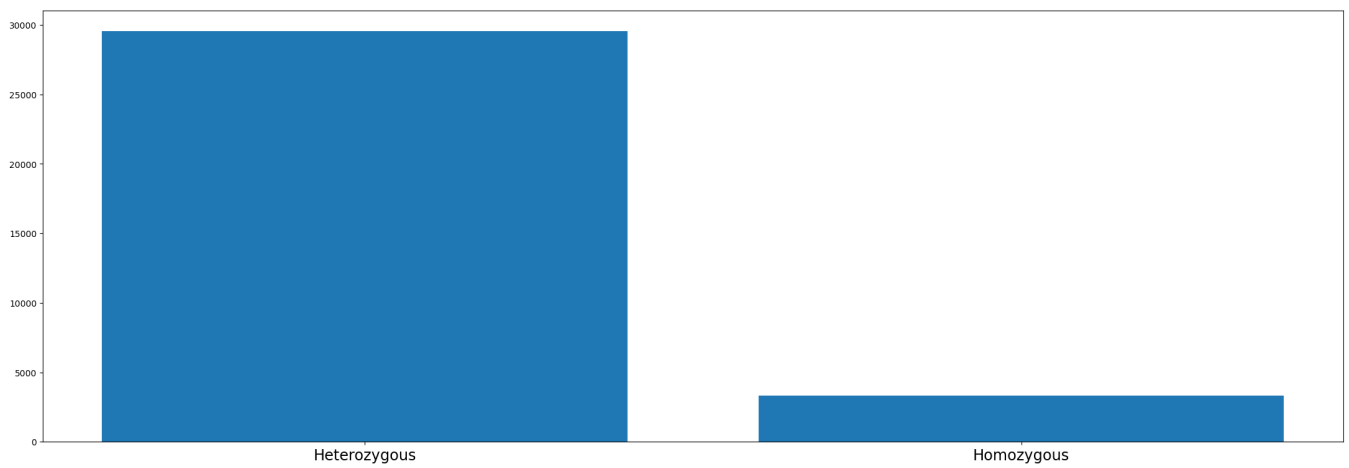
Figure 6: Feature distribution: d_b_hom.
