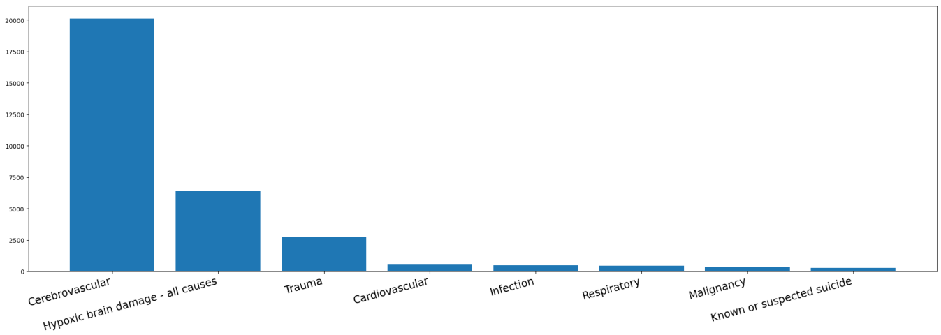
Figure 11: Feature distribution: dcod.
