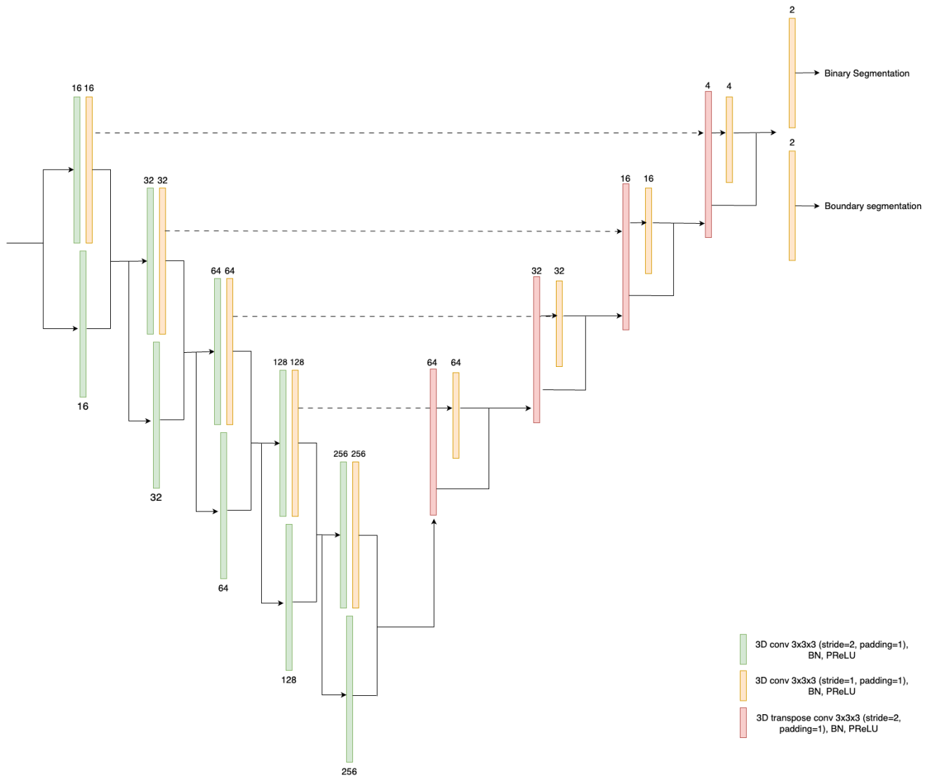
Figure 1. Network Architecture of the segmentation and boundary prediction model.
