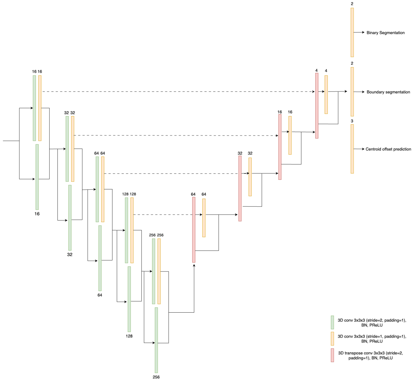
Figure 2. Network Architecture of the segmentation, boundary and offset model.
