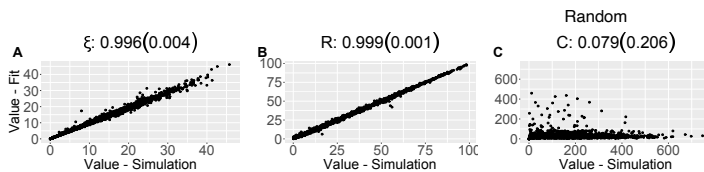
Figure S11: Parameter recovery scatter plot for Random model from \approx 100 simulations.
