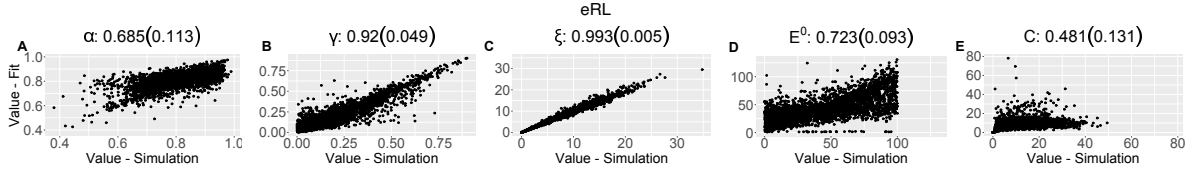
Figure S7: Parameter recovery scatter plot for eRL model from \approx 100 simulations.
