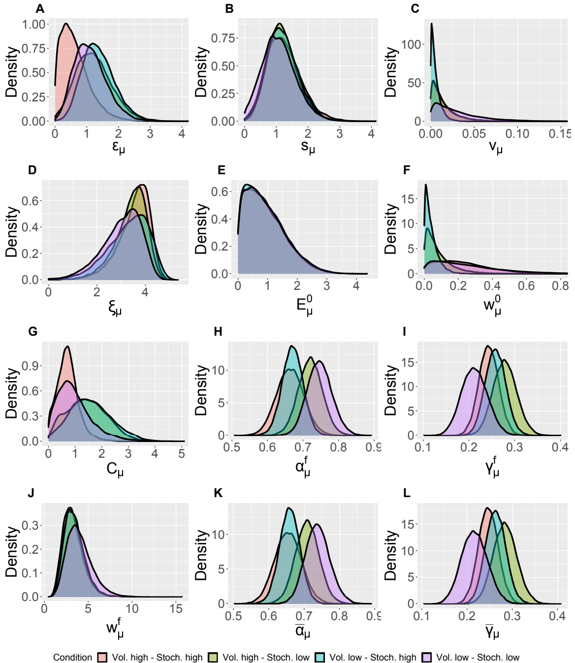
Figure S12: Group-level distributions for parameters for each condition for the eKF model.
