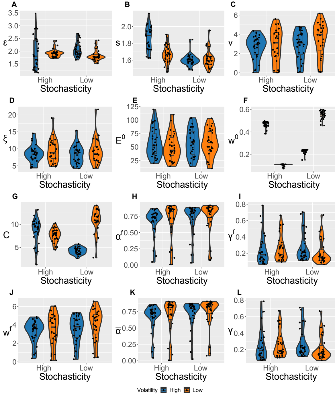
Figure S13: Violin plots (and box-plots) of individual-level parameters for each condition in the winning eKF model.
