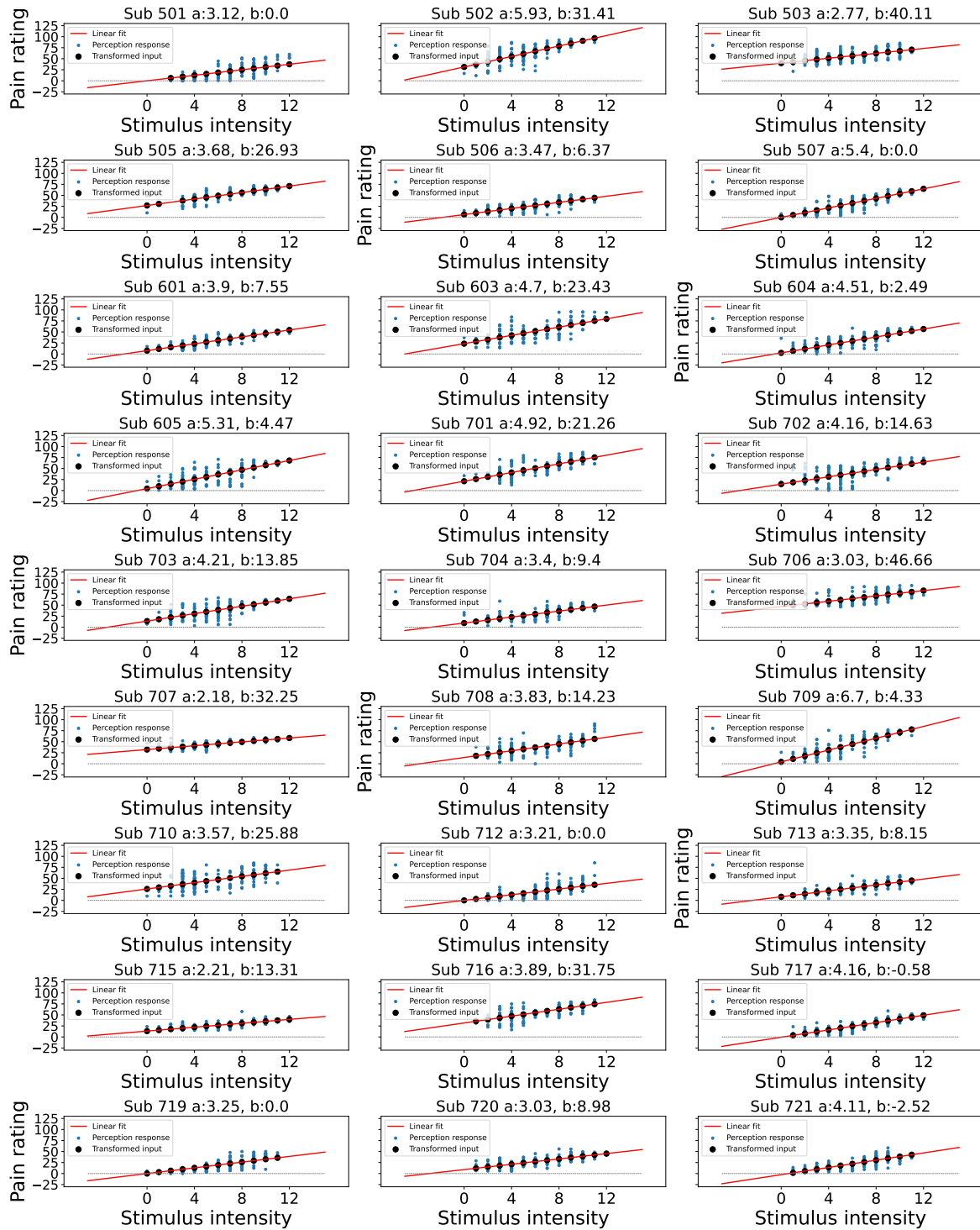
Figure S1: Linear transformation of the input at perception trials. Blue dots indicate participant's perception responses for a given level of stimulus intensity, black dots indicate transformed intensity values, a linear least squares regression was performed to achieve the best fitting line through participant responses as shown in red, the intercept was constrained >0 .
