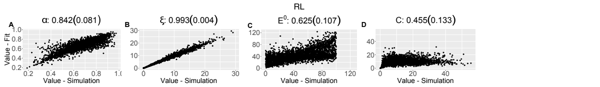
Figure S8: Parameter recovery scatter plot for RL model from \approx 100 simulations.
