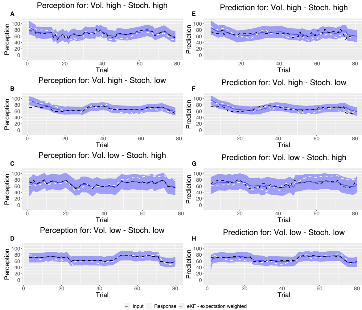
Figure S4: Example plot of the input sequences (black) for each condition, one participant's responses (white) and the winning, eKF, model predictions (blue) including 95% confidence intervals (shaded blue) for A-D : Perception and E-H : Prediction.
