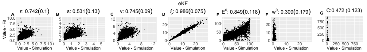
Figure S9: Parameter recovery scatter plot for eKF model from \approx 100 simulations.
