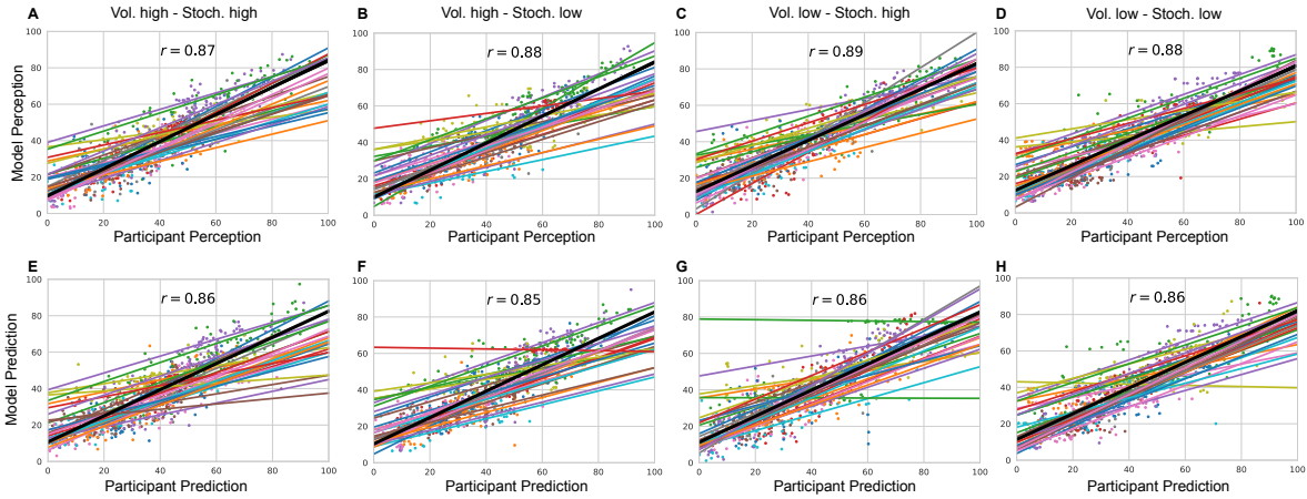
Figure S5: Model responses against participants responses for each condition and each response type A-D : Perception and E-H : Prediction. The annotated value is the grand mean correlation across subjects for each condition and response type.
