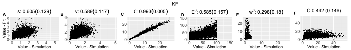
Figure S10: Parameter recovery scatter plot for KF model from \approx 100 simulations.
