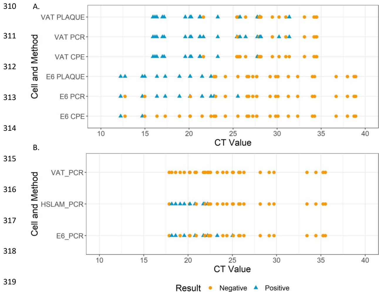
Figure 5. Positive and negative results by original Ct values using the different detection methods with A. Delta and B. Omicron samples, respectively. Each dot or triangle represents an individual sample. Most positive results were identified when samples had Ct < 25 regardless of the variant used. CPE: cytopathic effect, Plaque: plaque assay and PCR: RT-qPCR.
