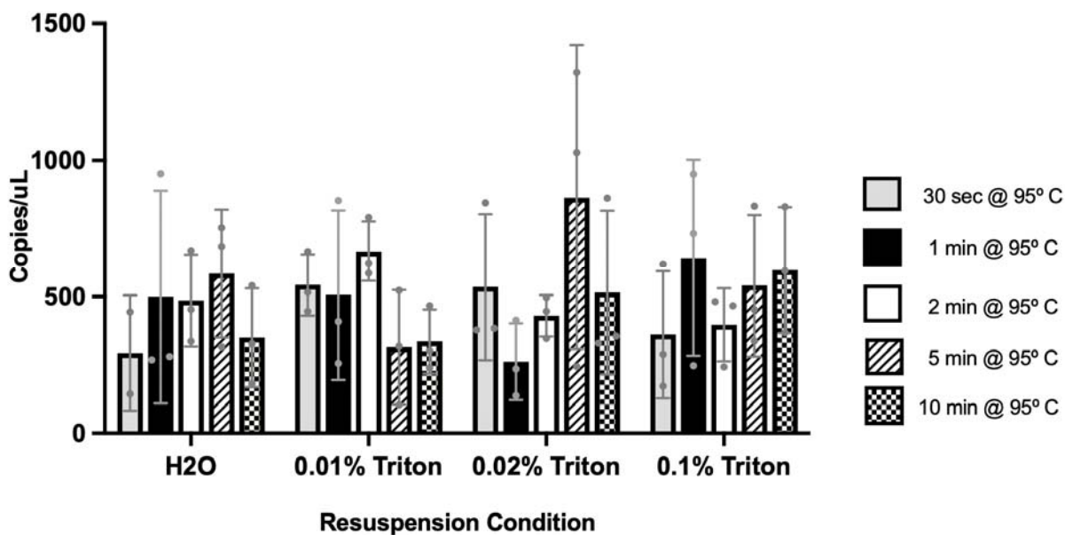
Figure 1 Legend: The figure shows copies per microliter of N. gonorrhoeae DNA that resulted from combination thermal and detergent extraction conditions. Dots represent distribution of data run in triplicate.
