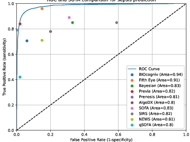
ROC and SOTA comparison for sepsis prediction
