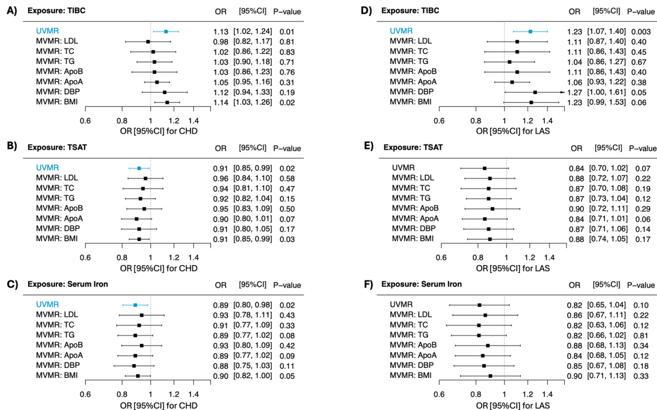
Figure 3. Associations between genetically predicted iron status and atherosclerotic cardiovascular disease outcomes using univariate and multivariate Mendelian randomization.
