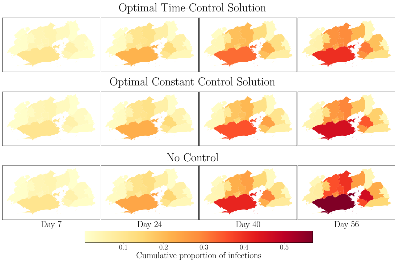
Figure 20: Disease Progression in the Rio de Janeiro Metropolitan Area under Various Vaccination Scenarios: This figure displays the cumulative proportion of infections via a heatmap, utilizing the framework established in Figure 18. Data sourced from Brazilian Institute of Geography and Statistics (IBGE) .
