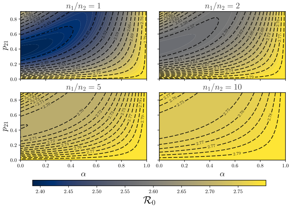
Figure 6: Basic reproduction number as function of \alpha and p_{21} for two cities: contour plot of the values of \mathcal{R}_0 for different values of \alpha \in (0, 1) , p_{21} \in (0, 0.9) and n_1/n_2 = (1, 2, 5, 10) considering \beta = (0.4, 0.1) .
