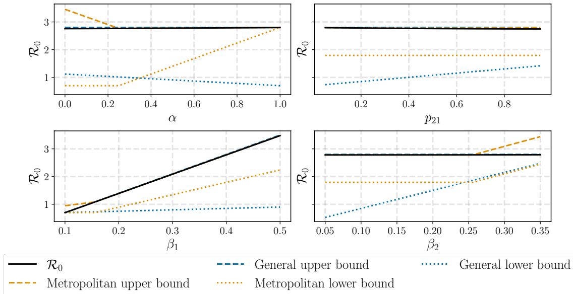
Figure 7: Impact of the parameters on the bounds of \mathcal{R}_0 : Using the same setting as in Figure 5, we visualize the impact of \alpha, p_{21}, \beta_1 and \beta_2 on \mathcal{R}_0 — depicted in black. In orange, we see the bounds from Theorem 2.2, and in blue, the bounds from Theorem 2.1. The dotted lines are the lower bounds while the dashed lines are the upper bounds.
