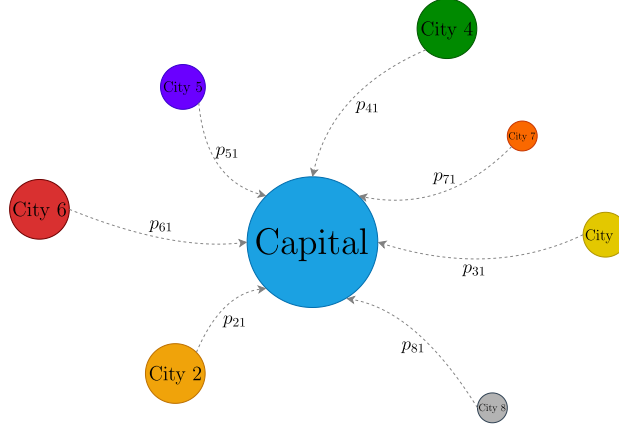
Figure 2: A version of Figure 1 considering a metropolitan area and the Assumption 2.1 .
