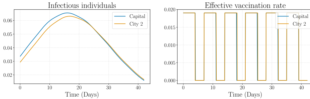
Figure 13: Optimal trajectories and control for two-city interaction for uniform infection rates: this figure shows the optimal trajectory of the proportion of susceptible and infectious individuals in two cities and the optimal control using the same settings as Figure 11 except for \beta = (0.25, 0.25) .
