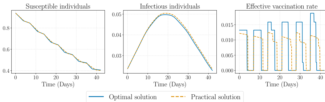
Figure 17: Comparison between optimal and practical solution in the metropolitan area: this figure presents the optimal trajectories and effective vaccination rate for the metropolitan area considering the settings of Figure 15. It compares the optimal solution with a more practicable solution, which is only based on the knowledge of vaccinated individuals. We observe that the effective vaccination rate here is the daily proportion of vaccinated individuals in the metropolitan area as a whole.
