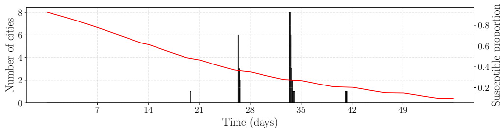
Figure 19: Analysis of Effective Vaccination Rates in the Rio de Janeiro Metropolitan Area: this figure presents two graphs – the red graph represents the proportion of susceptible individuals in Rio de Janeiro city, while the gray bars show the number of cities vaccinating when the capital is not. The settings of this experiment are identical to those in Figure 18 .
