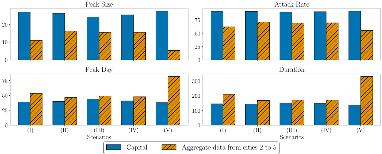
Figure 8: Simulation results for different structures of the transition matrix: comparison of Peak Size (maximum proportion of infectious individuals), Peak Day (day of the peak size), Duration (time from epidemic onset to the day when the proportion of infectious individuals achieves 10^{-5} ), and Attack Rate (proportion of individuals who contract the disease during 350 days of the epidemic) across different mobility scenarios. The aggregated data is the weighted average, considering their population size, from cities 2 to 5. For this experiment, \beta = (0.4, 0.25, 0.2, 0.15, 0.1) , \alpha = 0.64 and the population sizes are 10^5 \cdot (50, 10, 10, 1, 1) . Lastly, the initial conditions are I_1(0) = I_2(0) = I_3(0) = 10^{-4} and no recovered individuals.
