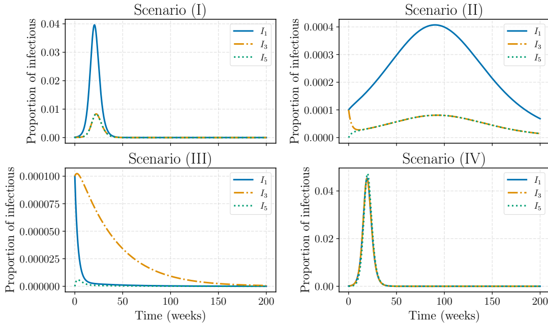
Figure 9: Infectious curves for different scenarios of \beta : this figure shows the curves of infectious individuals from cities 1, 3, and 5 under four different scenarios of the \beta specification. Here \alpha = 0.64 , p_{i1} = 0.2 for i \geq 2 and n_1 = 5n_2 = 5n_3 = 5n_4 = 5n_5 = 5 \cdot 10^6 . The four scenarios considered are (I) \beta = (0.2, 0.1, 0.1, 0.1, 0.1) , indicating \mathcal{R}_0^1 > 1 and \mathcal{R}_0^i < 1 for i \neq 1 ; (II) \beta = (0.15, 0.1, 0.1, 0.1, 0.1) , a situation similar to (I), but with a slower transmissibility rate, even though \mathcal{R}_0 > 1 ; (III) \beta = (0.1, 0.1, 0.15, 0.1, 0.1) , a situation similar to (II), but with the highest transmissibility rate not in the capital. This scenario results in \mathcal{R}_0 < 1 ; (IV) \beta = (0.2, 0.2, 0.2, 0.2, 0.2) , where all cities have the same transmissibility rate.
