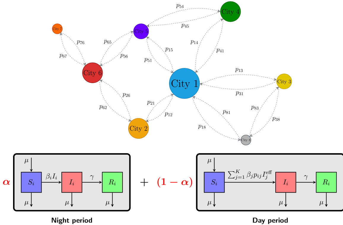
Figure 1: Graphical representation of city interactions and the SIR model: The cities are connected composing a network, p_{ij} being the proportion of individuals from city i who work during the day at j . At night, cities do not interact, and the epidemic follows a standard SIR dynamic. During the day, some individuals commute, interact with infected individuals in the destination city, and may transport the infection.
