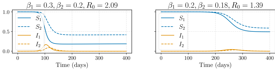
Figure 5: Dynamics of the Epidemic in Two Cities: epidemic dynamics in two cities under two different scenarios. The settings are \alpha = 0.64 , p_{21} = 0.2 and n_1 = 10 . The proportion of susceptible individuals is plotted in blue, and the proportion of infectious individuals in orange. The larger city is represented by a solid line, while the smaller city is represented by a dashed line. The basic reproduction number \mathcal{R}_0 , is calculated for each scenario.
