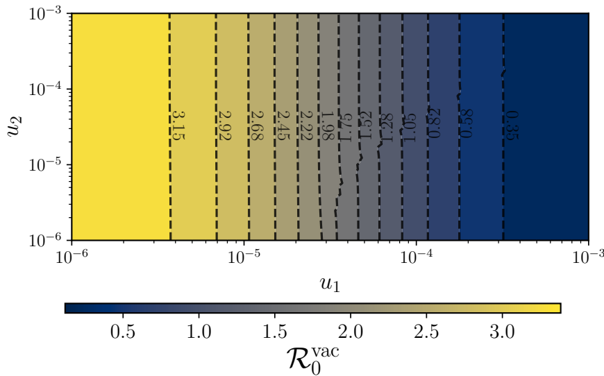
Figure 10: Basic reproduction number \mathcal{R}_0^{\text{vac}} in the vaccination model: this contour plot illustrates the basic reproduction number \mathcal{R}_0^{\text{vac}} for the model described in (5) as a function of u_1 and u_2 across K = 2 cities. The settings are: \beta = (0.5, 0.3) , \alpha = 0.64 , p_{21} = 0.2 and the ratio n_1/n_2 = 10 , similar to the settings in Figure 6. Both axes u_1 and u_2 are in the logarithmic scale.
