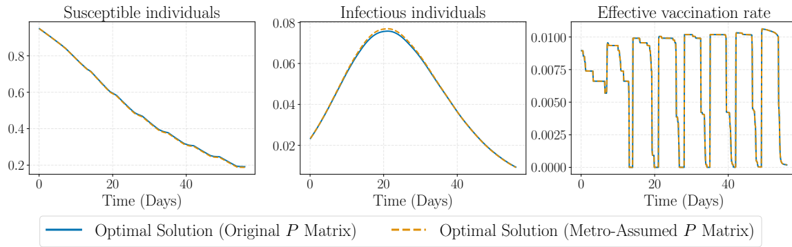
Figure 18: Comparative Analysis of Optimal Vaccination Strategies in the Rio de Janeiro Metropolitan Area: this figure illustrates the optimal vaccination strategies for Rio de Janeiro, through both the original and approximated P matrices. The settings are \alpha = 0.64 , a maximum vaccination rate of 0.6/56 per city, and weekly vaccine shipments for vaccinating up to 1/20 of the total susceptible population. The transmission rate \beta is randomly chosen between 0 and 0.3, and sorted by city population size. Vaccination starts when the susceptible population falls below 95% following the initial infection in the capital. The approximation of P in a metropolitan context is calculated by normalizing p_{i1} and p_{ii} by its sum.
