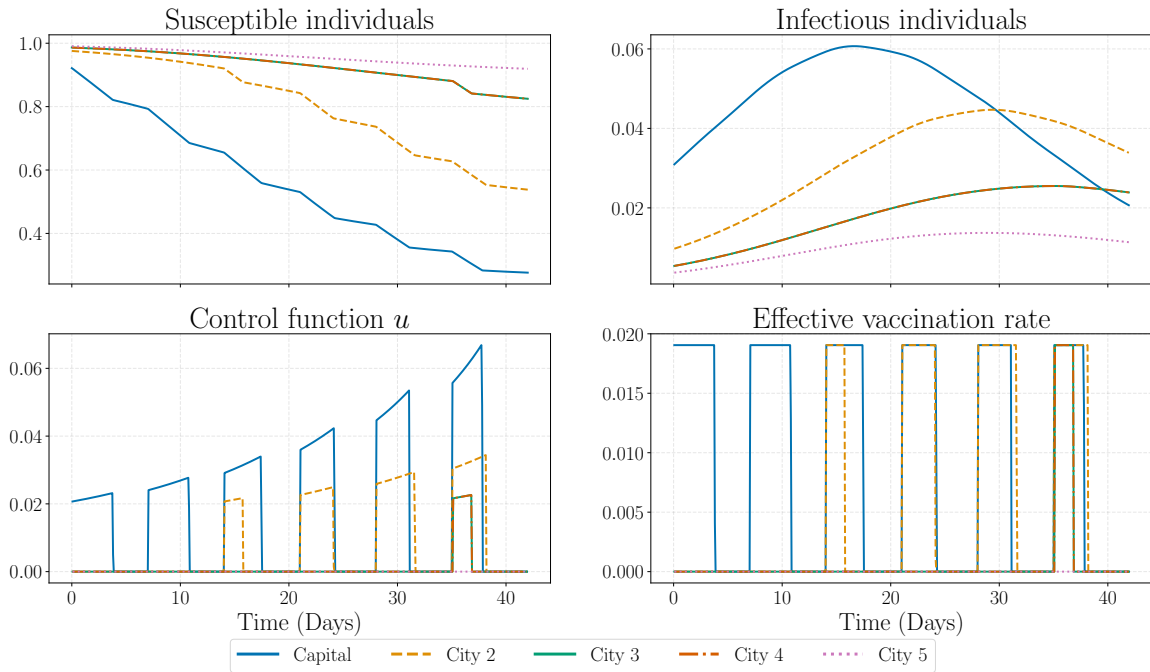
Figure 15: Optimal trajectories and control functions for 5 cities: this figure presents the optimal trajectories and controls for a problem involving 5 cities. The settings mirror those in Figure C.22a in the Appendix, with the following specifications: c_v = 0.01 , c_h = 1000 , and r_h = 0.1 . The model allows for a weekly vaccination of up to 1/20 of the susceptible population. The maximum rate of vaccinated individuals is set at v_1^{\max} = \dots = v_5^{\max} = 0.8/42 .
