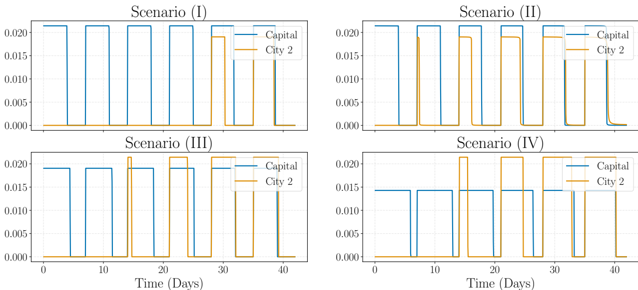
Figure 14: Optimal effective vaccination rate for two-city interaction: this figure shows four different scenarios. Scenario (I) considers the same setting as Figure 11 except for the first infection happening in the second city and v_1^{\max} = 0.9/42 (while v_2^{\max} = 0.8/42 ). Scenario (II) considers I_1(0) = I_2(0) = 0.05 and R_1(0) = R_2(0) = 0.02 . Scenarios (III) and (IV) fix the same parameters of Figure 11 but with different maximum rates v_1^{\max} and v_2^{\max} . In (III), we set v_1^{\max} = 0.8/42 < v_2^{\max} = 0.9/42 , while in (IV), v_1^{\max} = 0.6/42 < v_2^{\max} = 0.9/42 .
