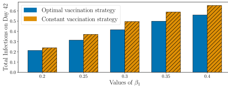
Figure 16: Comparison between optimal and constant vaccination strategies for different values of \beta_1 : this bar plot figure compares the total number of infections in the metropolitan area, which is calculated by integrating the new infections and taking the mean over the cities, for two scenarios. The first, in blue, solves the optimal control problem (9), and the second, in orange, chooses the best constant vaccination rate across all cities.
