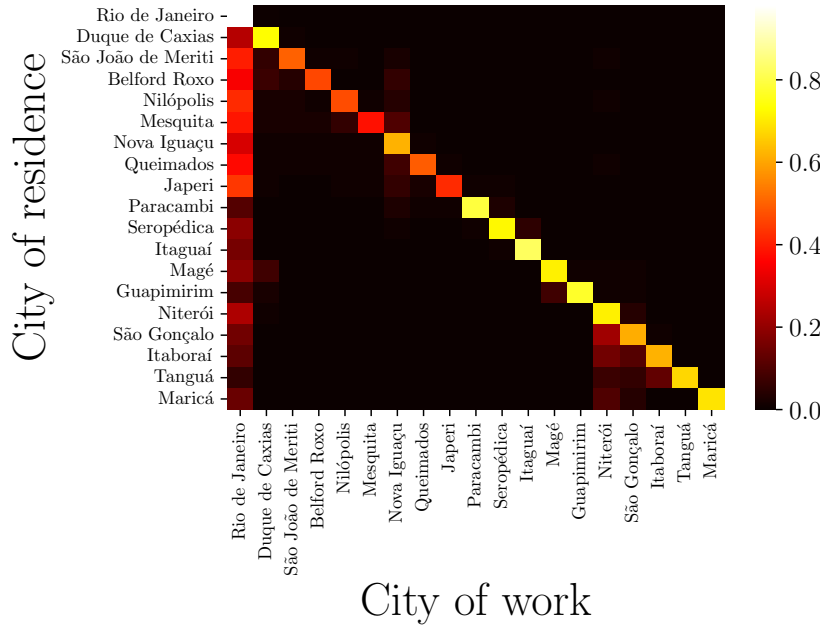
Figure 3: Transition matrix of the Rio de Janeiro metropolitan area: a heatmap showing the matrix P in the case of Rio de Janeiro metropolitan area (mobility data taken from [34]).
