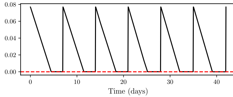
Figure 12: Weekly constraint analysis: this figure illustrates the function D(t) - \sum_{k=1}^K n_k V_k(t) for the experiment presented in Figure 11. In red, we fix the value 0 to give a reference.
