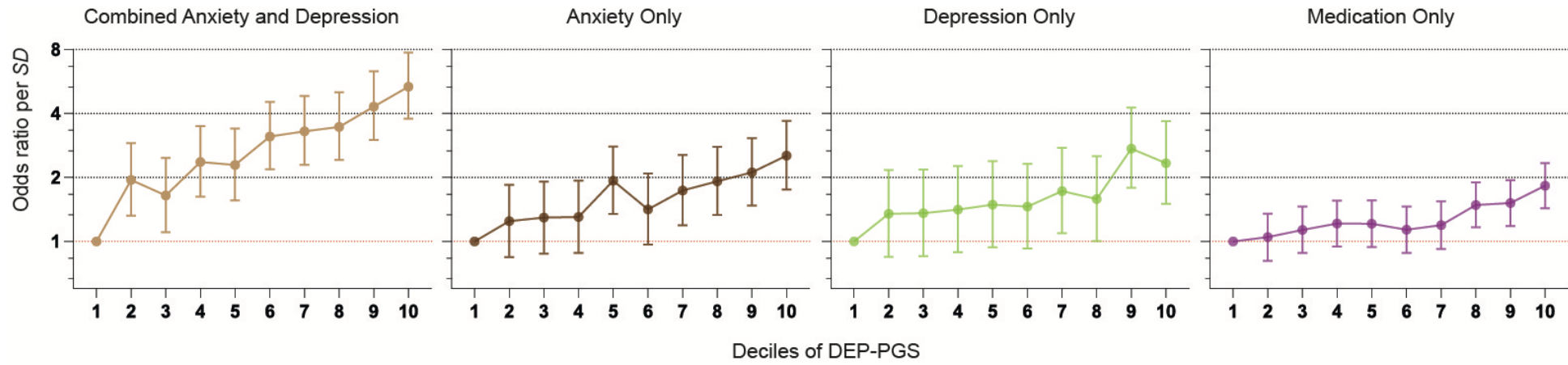
Figure 4. Genetic risk across the PGS distribution. OR per SD PGS with 95% CI for each decile of Depressive symptoms PGS (DEP-PGS) compared with the first decile.
