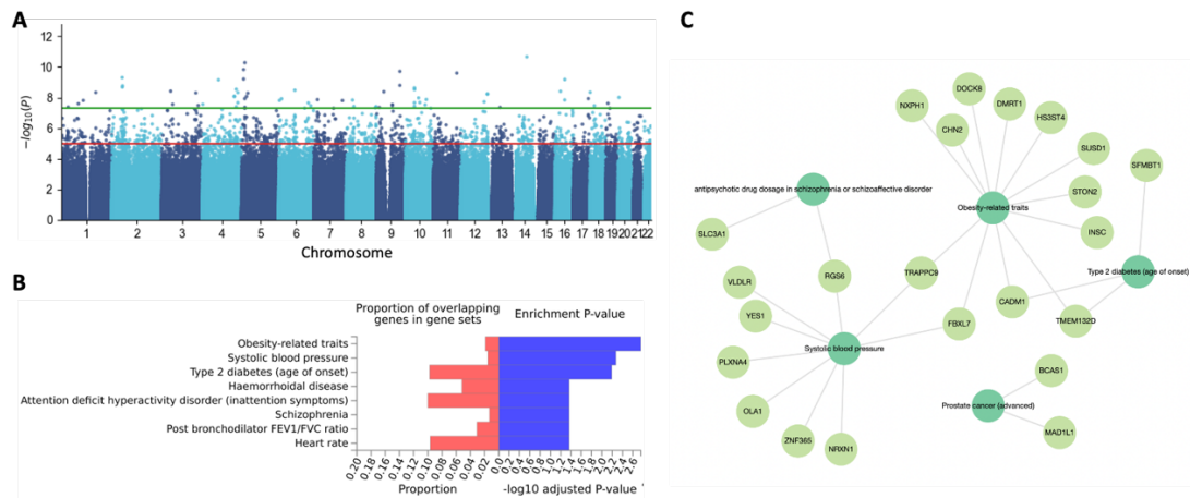
Fig. 2. GWAS results of \sim 10.2M variants for the IIH/PAP group. (A) Manhattan plot for Chr. 1 to Chr. 22. For visualization clarity we removed a single variant with extreme p-value ( rs12203577 , p-value 4.7E-70 ; Supplementary Table S3 ). The significant threshold of 5e-08 is depicted by the green horizontal line. (B) GWAS annotation enrichment of variants within the gene length based on the list of variants with p-value < 5e-07 (69 genes). Enrichment visualization for main GWAS results is based on GWAS-FUMA Gene2Func protocol. (C) Gene-phenotype network extracted from the results of GWAS catalog according to functional enrichment of EnriChR KB (see Methods).
