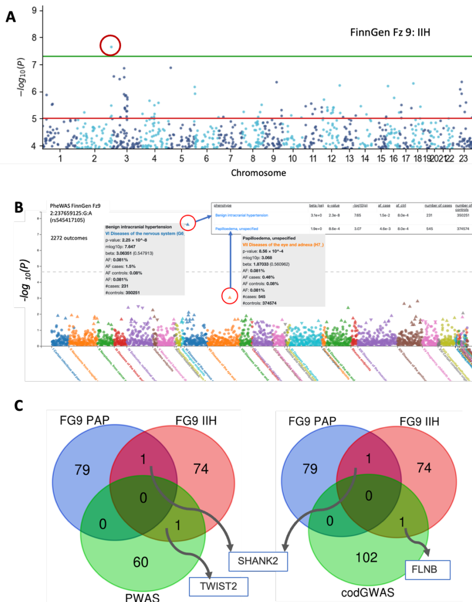
Fig. 5. FinnGen Fz9 results for IIH associations. (A) Manhattan plot of the results from FinnGen Fz9 for Benign intracranial hypertension (named G6_BENINTRAHYP). The significant variant in Chr. 2 is marked by a red circle. For fine mapping analysis see Supplementary Fig. S4 . (B) PheWAS results for variant 2:237659125:G:A (rs545417105). All phenotypes (with 2272 codes) are clustered by their medical relevance (color coded). The triangle pointing up and down indicate an increase or decrease in the risk for the relevant disease, respectively. The most significant phenotypes were associated with an increased risk for IIH and
