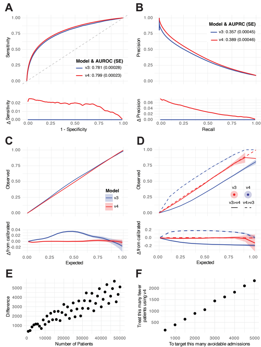
Figure 2: Comparison of overall predictive performance between SPARRA v3 and SPARRA v4 . (A) ROC. (B) PRC. Lower sub-panels show differences in sensitivity and precision, respectively. Confidence intervals are negligible. (C) Calibration curves. (D) Calibration curves for samples in which |v4 - v3| > 0.1 . Lower sub-panels show the difference between curves and the y = x line (perfect calibration). Confidence envelopes are pointwise (that is, for each x -value, not the whole curve). Predicted/true value pairs are combined across cross-validation folds in all panels for simplicity. (E) Difference in the number of individuals who had an event amongst individuals designated highest-risk by v3 and v4 . The repeating pattern is a rounding effect of v3 . (F) Difference in the number of highest-risk individuals to target to avoid a given number of admissions.
