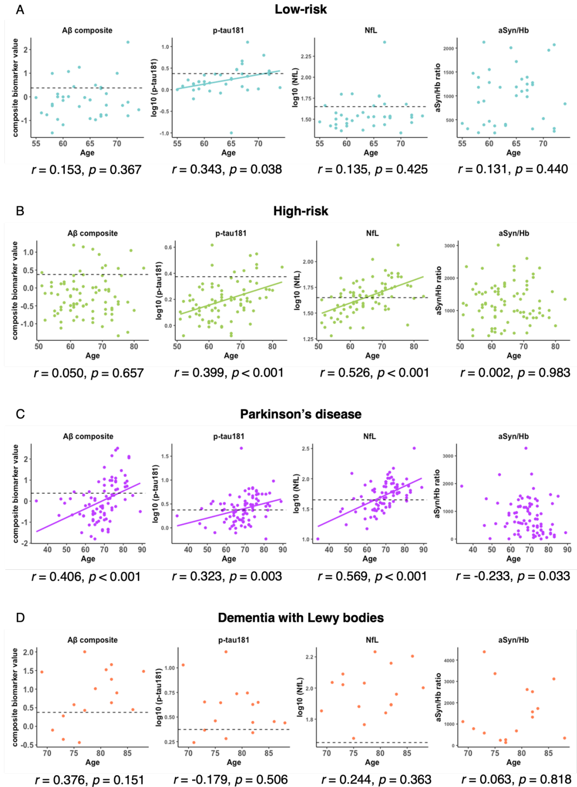
Supplementary Figure 1. Pearson's correlation between plasma biomarkers and age Pearson's correlation test between plasma biomarkers and age in the low-risk group (A), high-risk group (B), Parkinson's disease group (C), and dementia with Lewy bodies group (D). The
