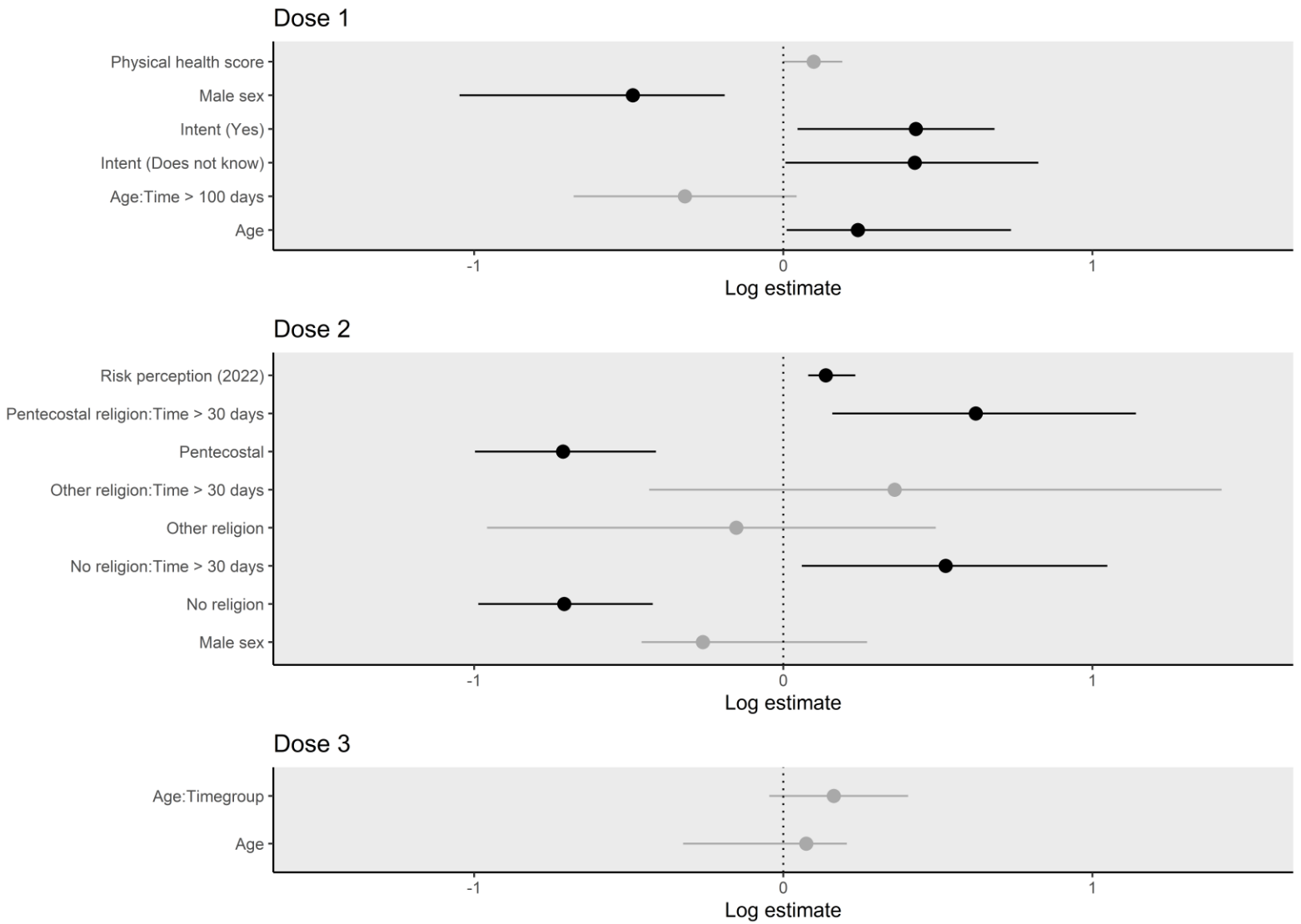
Figure 4: Model results.
