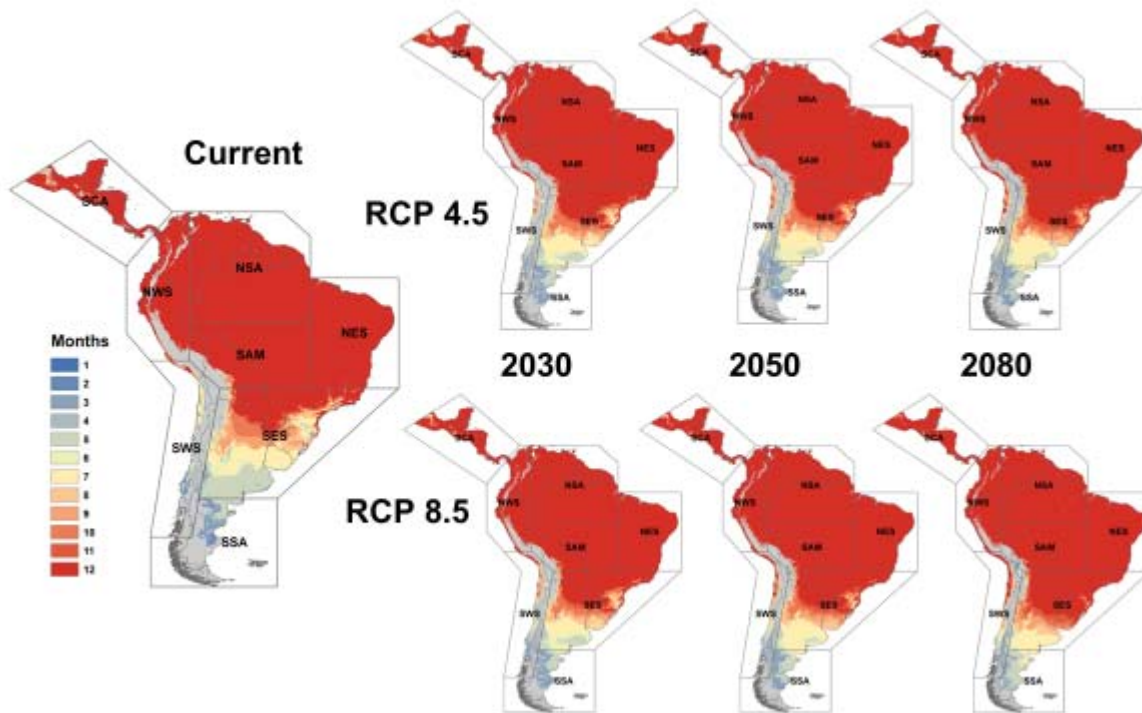
327 328 Fig. 6. Thermal suitability for transmission of Plasmodium falciparum malaria by the potential 329 invasive Anopheles stephensi . 330
