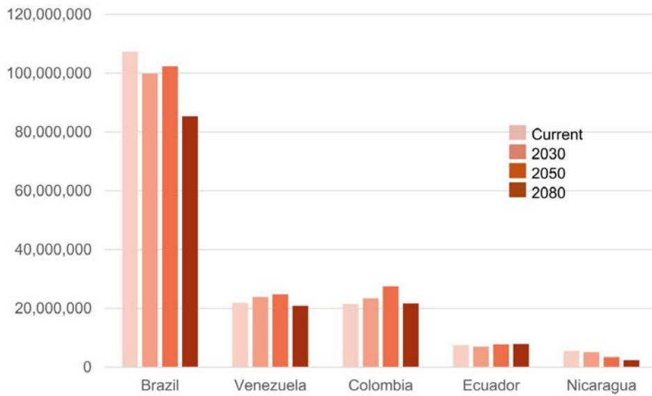
355 Fig. 8. Top five countries in Central and South America with the highest population at risk (PAR) 356 for exposure to year-round P. falciparum malaria (A) and P. vivax malaria (B) transmitted by the 357 potential invasive An. stephensi . PAR will change in the future as geographic suitability shifts 358 under climate change (RCP 4.5 shown). 359
