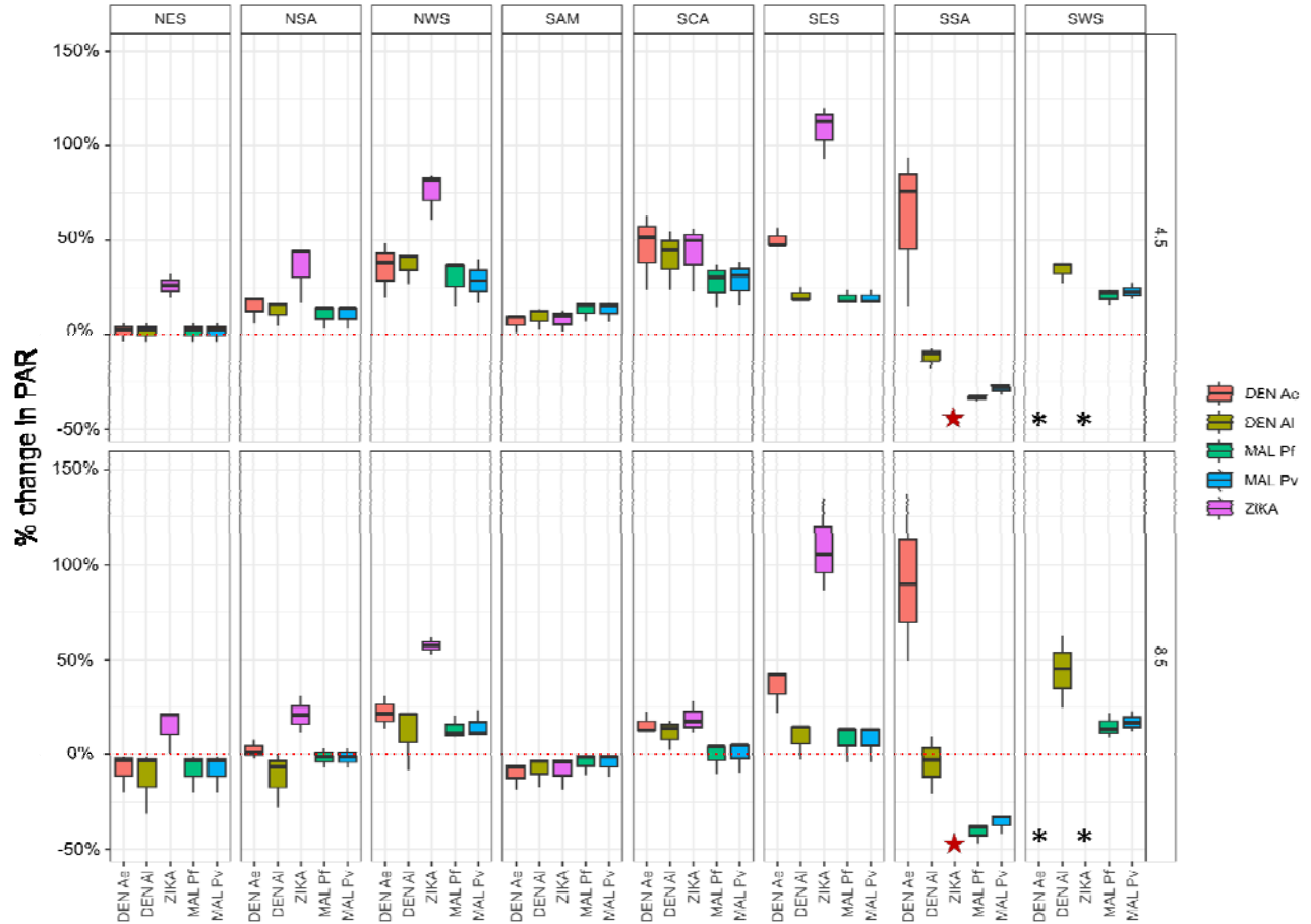
249 Figure 2. The percent of change in people at risk (PAR) from baseline to 2030, 2050, 2080 250 (given as boxplot) under the two climate projections, RCP 4.5 and RCP 8.5, for the five potential 251 MBDs in this study, across the 8 sub-regions of Central and South America defined by IPCC for 252 one or more months of suitability. DEN Ae = dengue transmitted by Aedes aegypti ; DEN Ai = 253 Dengue transmitted by Aedes albopictus ; MAL Pf = Plasmodium falciparum malaria transmitted 254 by Anopheles stephensi ; MAL Pv = P. vivax malaria transmitted by An. stephensi ; ZIKA = Zika 255 virus transmitted by Ae. aegypti . Note: at baseline there is no predicted risk for ZIKA in SSA, so 256 all change is infinite (red star); SWS, changes exceeded 150% for DEN Ae and ZIKA (black 257 asterisks).
