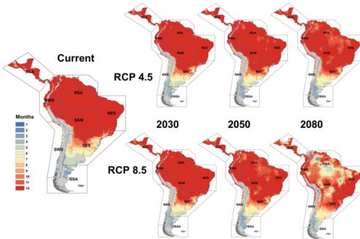
351 352 Fig. 7. Thermal suitability for transmission of Plasmodium vivax malaria by the potential invasive 353 Anopheles stephensi .
