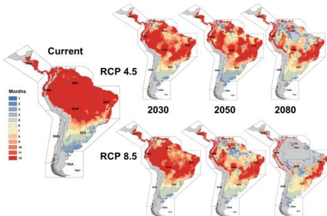
281 Fig. 3. Thermal suitability for dengue transmitted by Aedes albopictus .
