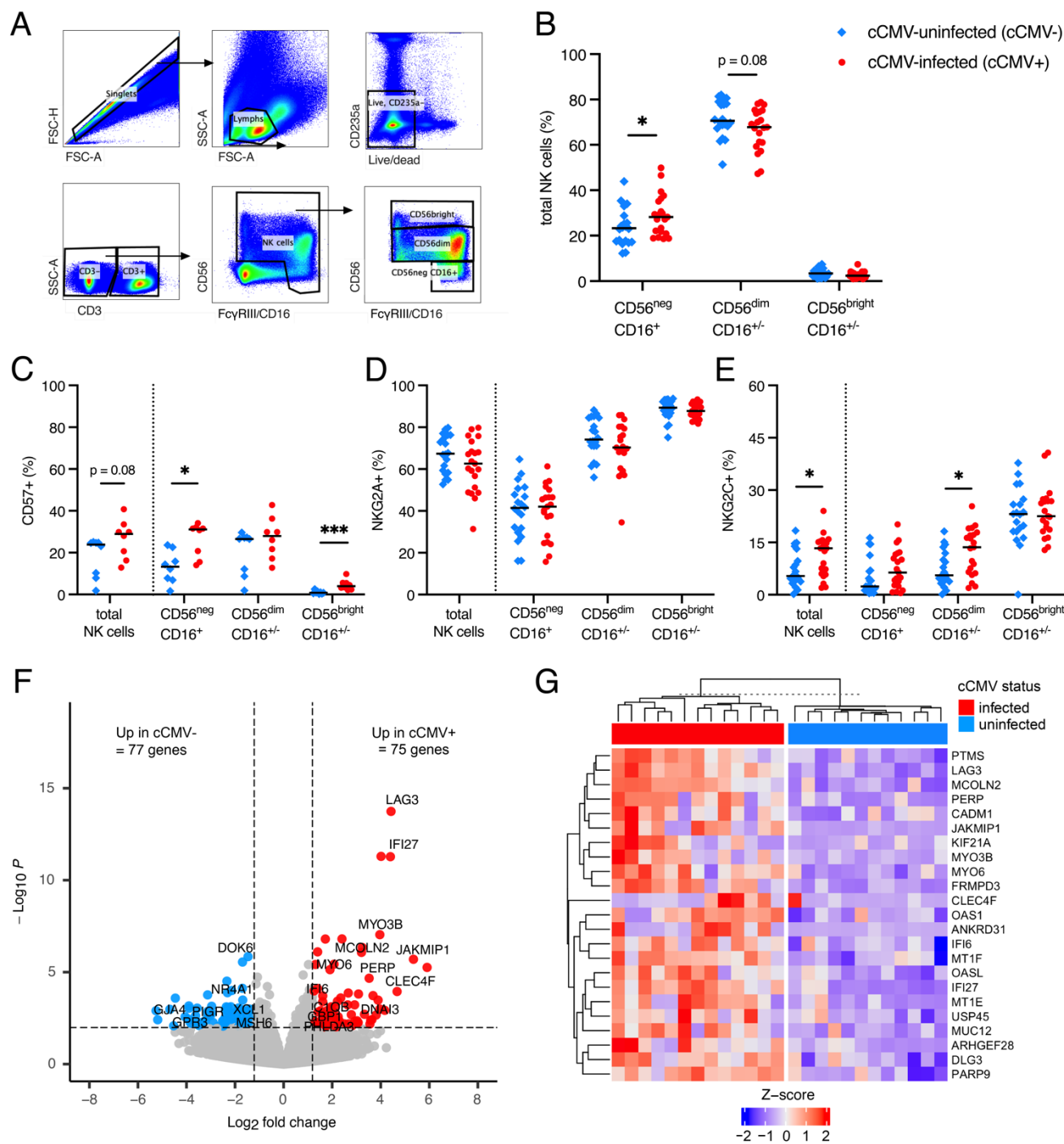
Figure 2. CD16/FcyRIII + CD56 neg and NKG2C + NK cells expand in cord blood from cCMV-infected versus cCMV-uninfected neonates. NK cell immunophenotypes and transcriptional profiles were compared in umbilical cord blood from cCMV-infected (cCMV+, red circles) versus cCMV-uninfected (cCMV-, blue diamonds) neonates. (A) NK cell gating strategy. (B) Frequencies of NK cell subsets in cCMV+ (n=21) versus cCMV- (n=20) neonates. (C) Frequency of total NK cells and NK cell subsets expressing CD57 in cCMV+ (n=8) versus cCMV- (n=8) neonates. (D-E) Frequency of total NK cells and NK cell subsets expressing (D) NKG2A and (E) NKG2C in cCMV+ (n=21) versus cCMV- (n=20) neonates. (F) Volcano plot demonstrating differentially expressed genes in FAC-sorted total NK cells from cCMV+ (n=13) and cCMV- (n=12) neonates. Significance was set at P < 0.01 and \log_2 foldchange \pm 1.2 . Red circles indicate genes enriched in cCMV+ NK cells, blue circles indicate genes enriched in cCMV- NK cells, and grey circles indicate genes whose expression did not differ significantly between groups. (G) Heatmap of top 23 enriched genes (FDR P < 0.1 , \log_2 foldchange > 1.2 ) in NK cells from cCMV+ (n=13) versus cCMV- (n=12) neonates. Z-score shows gene expression based on \log_2 -transformed data. FDR-corrected P values for Mann-Whitney U test. * P < 0.05 , ** P < 0.01 , *** P < 0.001 .
