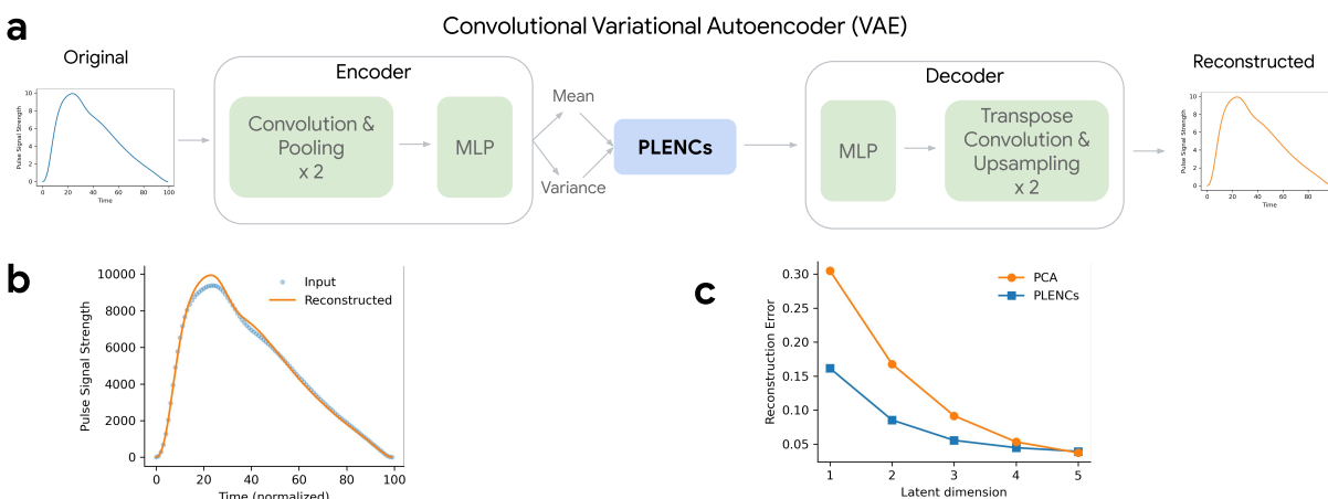
Figure 3: Overview of REGLE on PPG. a) Learning PPG encodings (PLENCs) using a convolutional variational autoencoder (VAE). b) Reconstructing PPG from PLENCs (dim=5). c) Reconstruction errors (mean squared error across time points) for reconstructed PPGs using the PLENCs model and PCA with a varying latent dimension. Both the PLENCs model and PCA are trained (or “fitted”) on a training set and the reconstruction error was evaluated in a separate validation set.
