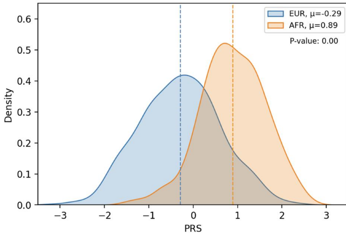
Fig 1. Density plot of PRS distributions by ancestry, normalized to entire population. The EUR curve represents European ancestry. The AFR curve represents African ancestry.
