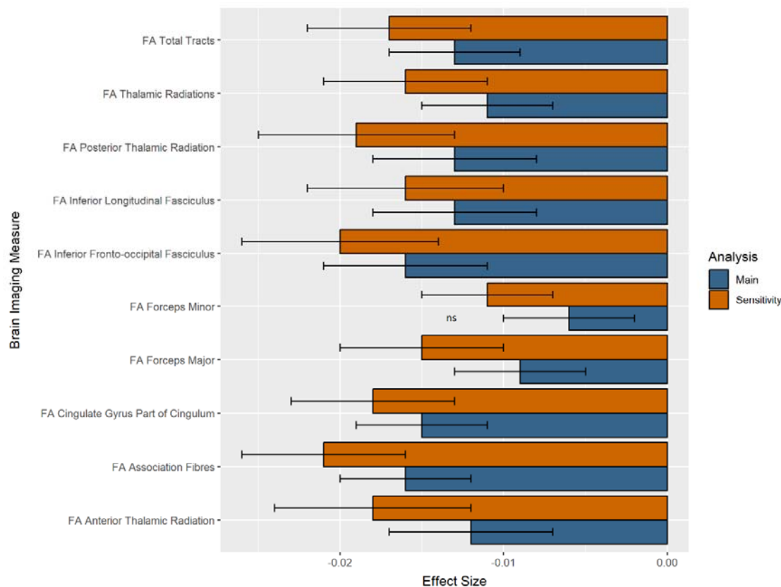
Fig 2. Standardised effect sizes for white matter microstructure neuroimaging measures associated with seasonality in the main and sensitivity analyses. All shown measures were associated with seasonality ( p_{corr} < 0.05 ), except for FA Forceps Minor in the main analysis (ns = non-significant).
