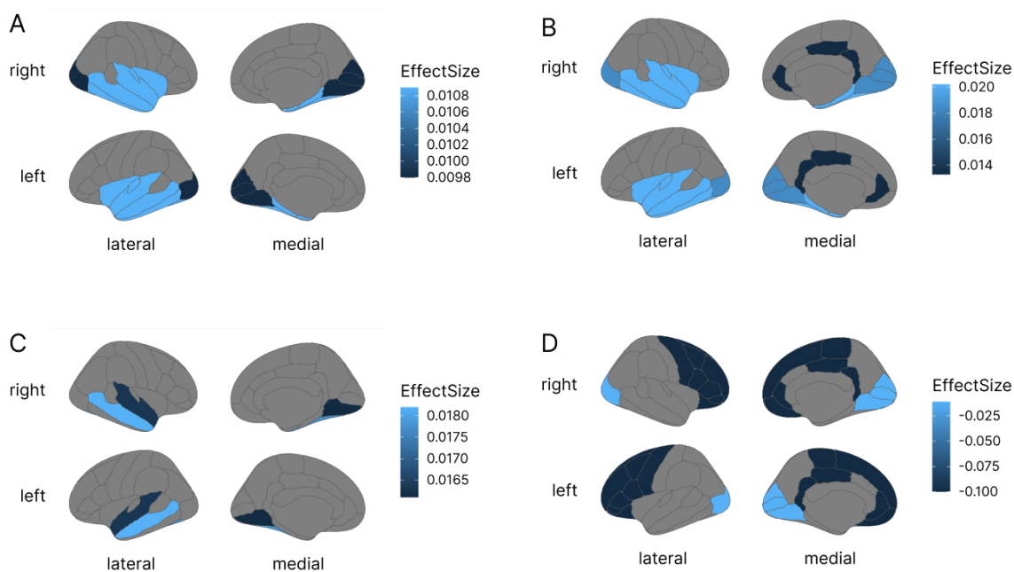
Fig 1. Standardised effect sizes of brain morphology measures associated with seasonality mapped onto the Desikan-Killiany-Tourville atlas for (A) mean cortical thickness of the temporal and occipital lobes in the main analyses and in the sensitivity analyses for (B) mean cortical thickness of the middle temporal, fusiform, superior temporal and lingual gyri, (C) mean cortical thickness of the temporal, occipital and cingulate lobes, and (D) cortical surface area of the frontal, occipital and cingulate lobes. Darker colour indicates associations with winter births, lighter colour indicates associations with summer births.
