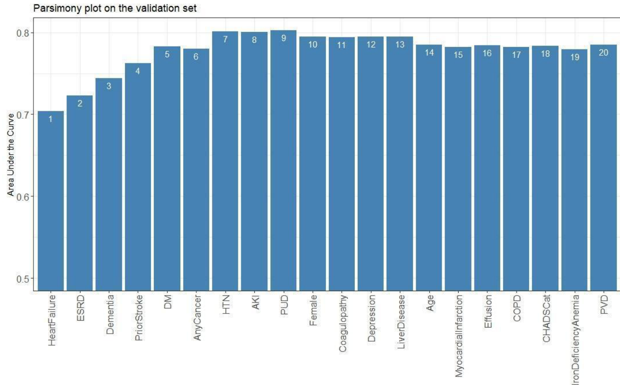
Figure 2. Parsimony plot of the new model's performance predicting stroke (as indicated by the area under the curve) as a function of the model's complexity (as noted in the number of variables included in the model). The AUC (accuracy of the model) increased with the addition of variables till HTN; no further increase in accuracy could be achieved with the addition of other variables beyond variable 8 (AKI). This indicates that the model's highest accuracy was attained with the first seven variables.
