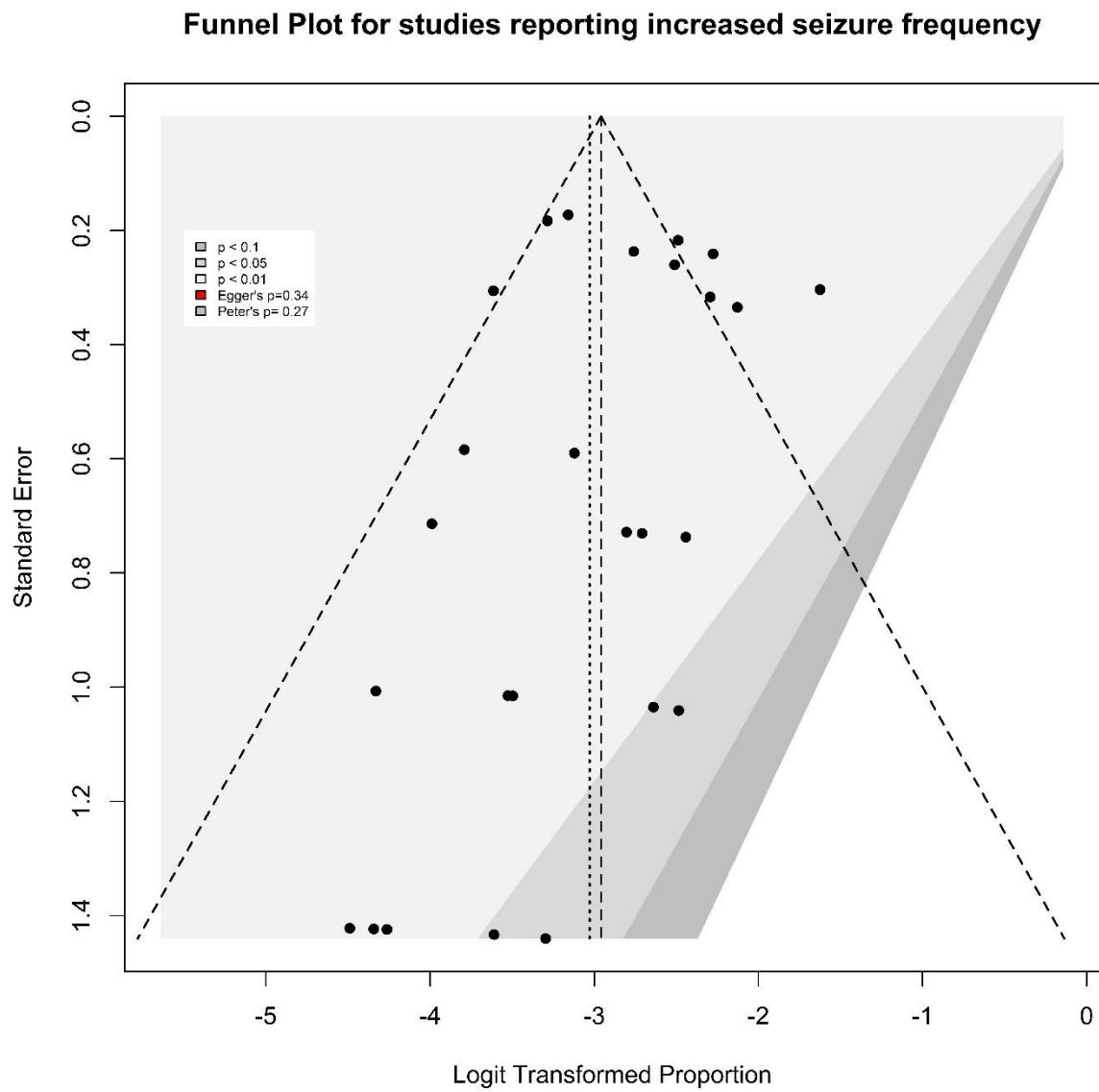
Figure S2- Funnel plot for studies reporting increased seizure frequency after COVID-19 vaccines.
