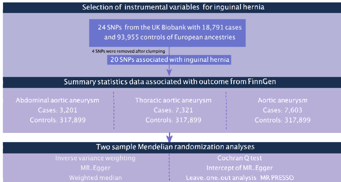
Figure.1 Study overview of this mendelian randomization.
