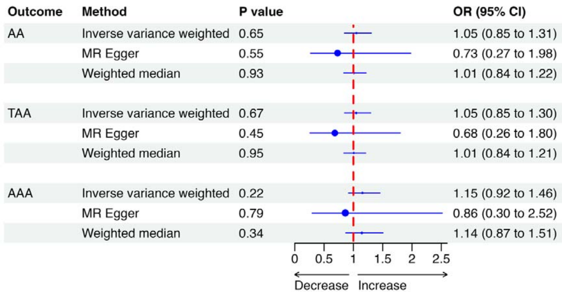
Figure.2 Results of three different mendelian randomization methods to investigate genetic association between inguinal hernia and aortic aneurysms. Abbreviations: MR, mendelian randomization; AA, aortic aneurysm; TAA, thoracic aortic aneurysm; AAA, abdominal aortic aneurysm; CI, confidence interval; OR, odds ratio.
