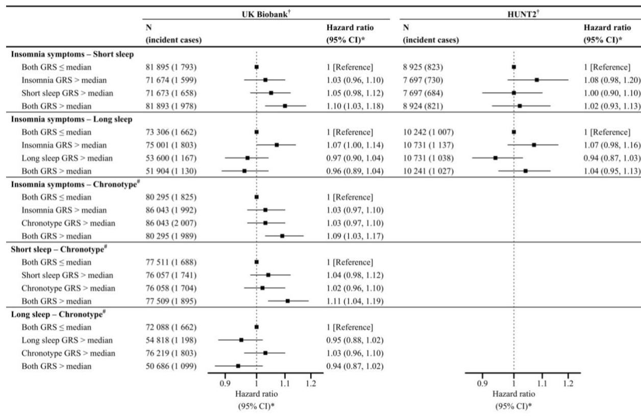
Figure 2: 2x2 factorial Mendelian randomization Cox regression analysis assessing the joint effects of two sleep traits with risk of incident acute myocardial infarction in UK Biobank and HUNT2
