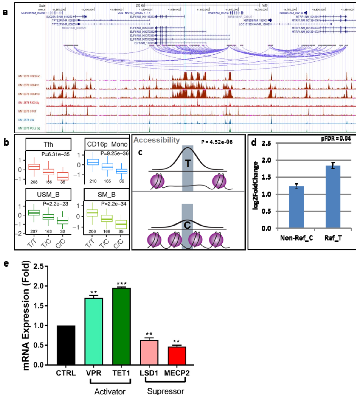
Figure 3. Analysis of LOC_125. This locus has two index SNPs and 15 high-LD SNPs. Of these, rs57668933 is a caQTL-SNP and has allele-specific enhancer activity. a) Visualized connections of rs57668933 and neighboring regions based on PCHiC, alongside various histone marks. b) The SNP lies in ELF1 , a significant eQTL gene. Significant genotype-specific gene expression in follicular T-helper cells (Tfh), CD16 + monocytes, and unstimulated and stimulated B-cells; c) chromatin accessibility of alleles. Reference allele T has higher chromatin accessibility. d) MPRA data shows T has higher enhancer activity. e) CRISPR-dCas9-based targeting of rs57668933-containing region by two activators (dCas9-VPR and dCas9-TET1) and two suppressors (dCas9-MECP2, dCas9-LSD1) and ELF1 (target gene) mRNA expression.
