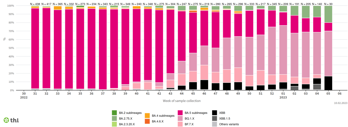
Figure S1: Distribution of sequenced Omicron lineages in Finland The graph shows the percentages of the most frequent SARS-CoV-2 sublineages detected by sentinel surveillance and recorded in the National Infectious Diseases Register by week of sample collection since August 2022. Green bars represent BA.2 sublineages (BA.2 lineages, BA.2.75.X and BA.2.3.20.X), orange bars represent BA.4 sublineages (BA.4 lineages and BA.4.6.X) and pink bars represent BA.5 sublineages (BA.5 lineages, BF.7.X and BQ.1.X). The black bars represent sublineages that descended from the XBB recombinant lineage and the group ‘Other variants’ represents sublineages not assigned to any of the previous groups. The .X extension covers the whole sublineage family, e.g. BQ.1.X covers all descendants of BQ.1, such as BQ.1.1 and BQ.1.2.
